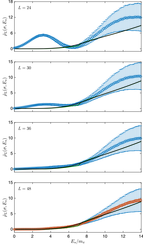
FIG. 14. Reproduction of Fig. 9 using the smaller value \sigma = 0.075 of the smearing parameter. As expected, in the first row the peak becomes sharper, and in all cases the error increases at high energy due to larger systematic uncertainties.
