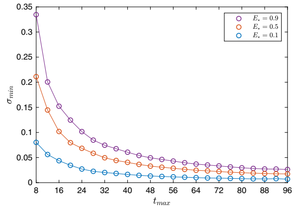
FIG. 4. Solution to the equation \delta_{\sigma}(E_{\star}, E_{\star}) = 0.05 as a function of t_{\max} for three different values of E_{\star} in the case where B[g] = 0 . The solution indicates the smallest possible choice of \sigma that ensures that the relative error on the target smearing function is below 5%.
