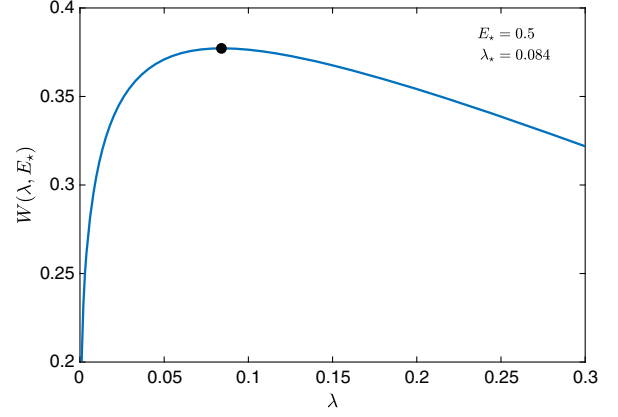
FIG. 5. The function W(\lambda, E_\star) in the case of the lattice QCD correlator discussed in section V at E_\star = 0.5 . This function has a characteristic shape exhibiting a maximum at the optimal value \lambda_\star of the trade-off parameter where the deterministic and error functionals are equally important in the minimization procedure.
