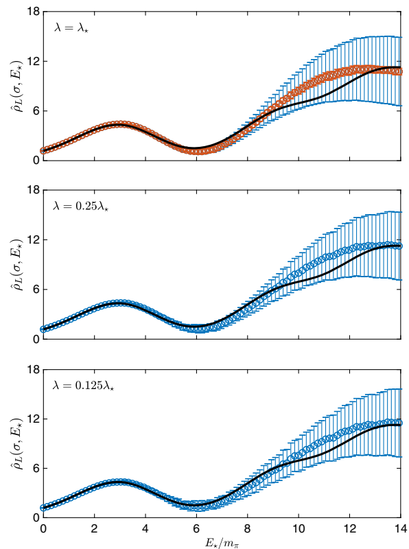
FIG. 7. Examples of how the reconstructed spectral density depends on the \lambda parameter. In the topmost plot, the orange band shows the statistical uncertainty, while in all cases the blue band shows the combined uncertainty (statistical and systematic). For this particular case, where L = 24 and t_{\max} = 30 with \sigma = 0.1 , the dependence on \lambda is practically negligible. These results have been obtained by using b_\infty(t, E) as basis functions.
