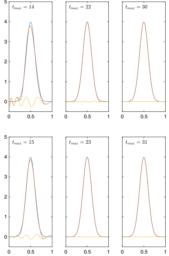
FIG. 3. Comparison of the target smearing function \Delta_{\sigma}(E_{\star}, E) (blue curves) at E_{\star} = 0.5 and \sigma = 0.1 with the functions \tilde{\Delta}_{\sigma}(E_{\star}, E) (red curves) obtained with our method. In each row the different panels correspond to different values of t_{\max} . The panels in the first row correspond to the choice of b_{\infty}(t, E) as basis functions while the panels in the second row correspond to the choice of b_T(t, E) with T = 2(t_{\max} + 1) . In all plots the yellow curve shows the difference, and as expected, it goes to zero in the limit of large t_{\max} .
