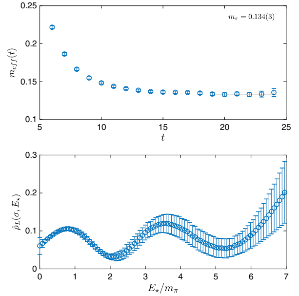
FIG. 10. Extraction of the smeared spectral density from the correlator C_{\text{QCD}}(t) discussed in the text. The top panel shows the calculation of the pion mass, the lightest state contributing to the spectral density in this case, extracted from a standard effective-mass analysis. The bottom panel shows the reconstructed smeared spectral density obtained by applying our method with \sigma = 0.1 , by using b_T(t, E) as basis functions with T = 48 = (2t_{\text{max}} + 1) , by setting E_0 = 0.37m_\pi and by using the value of \lambda_* determined at E_* = 3.7m_\pi for all the energies explored. As expected, the smeared spectral density shows a peak in correspondence of E_*/m_\pi \simeq 1 and another structure around E_*/m_\pi \simeq 3 .
