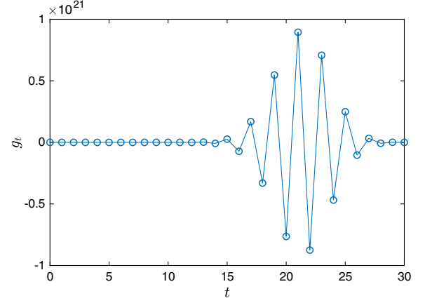
FIG. 2. Values of the coefficients g_t(E_\star) corresponding to the smearing function \Delta^{\text{BG}}(E_\star, E) shown in the right panel of Fig. 1, i.e., the coefficients obtained by applying the Backus-Gilbert procedure in the absence of statistical errors with E_\star = 0.5 , b_\infty(t, E) as basis functions and t_{\max} = 30 . A typical pattern for these coefficients is that they change sign and for some values of t they have extremely large absolute values (the scale on the y axis varies between \pm 10^{21} ).
