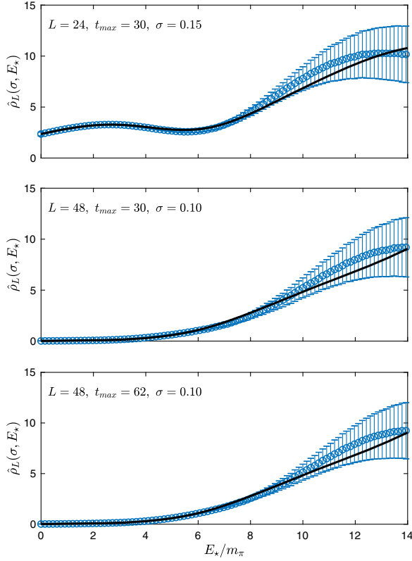
FIG. 8. In cases where the smeared spectral density is very smooth, either because the smearing parameter \sigma is larger (top-most plot), or because we are closer to the infinite-volume result (second and third plots), the quality of the reconstruction is much better. For the second and third plots we use two different values of t_{\max} , and while increasing t_{\max} does improve the result slightly, already at t_{\max} = 30 we have full control over the reconstruction of the spectral density. These results have been obtained by using b_\infty(t, E) as basis functions.
