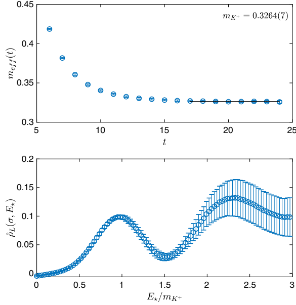
FIG. 11. Extraction of the smeared spectral density from the correlator C_{\text{QCD+QED}}(t) discussed in the text. The top panel shows the calculation of the charged kaon mass, the lightest state contributing to the spectral density in this case, extracted from a standard effective-mass analysis. The bottom panel shows the reconstructed smeared spectral density obtained by applying our method with \sigma = 0.1 , by using b_T(t, E) as basis functions with T = 48 = (2t_{\text{max}} + 1) , by setting E_0 = 0.15m_{K^+} and by using the value of \lambda_* determined at E_* = 1.5m_{K^+} for all the energies explored. As expected, the smeared spectral density shows an isolated peak in correspondence of E_*/m_{K^+} \simeq 1 and another structure that starts in proximity of E_*/m_{K^+} \simeq 2.4 .
