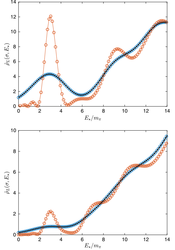
FIG. 6. Comparison of the results obtained with our method (blue points) with the results obtained by using the Backus-Gilbert method (orange points) in the absence of statistical errors. The two plots correspond to the volumes L = 24 (first row) and L = 32 (second row) with t_{\max} = 30 in both cases. In the case of our method the results have been obtained by setting E_0 = 0 and by using the Gaussian of Eq. (24) as the target smearing function with \sigma = 0.1 . In both plots the solid black curve corresponds to the exact smeared spectral density that our method (not the Backus-Gilbert one) is expected to reproduce in the infinite- t_{\max} limit.
