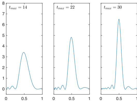
FIG. 1. Smearing functions \Delta^{\text{BG}}(E_\star, E) obtained by applying the Backus-Gilbert procedure in the absence of statistical errors with E_\star = 0.5 and b_\infty(t, E) as basis functions. The different panels correspond to different values of t_{\max} . As it can be seen the function \Delta^{\text{BG}}(E_\star, E) gets more similar to a Dirac \delta function for increasing values of t_{\max} .
