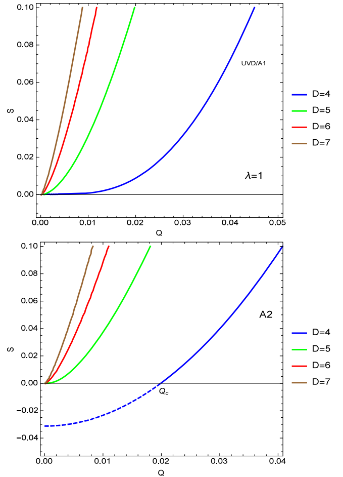
FIG. 6. Qualitative behaviors of the curves of extreme BHs in the Q-S plane for the three families of central-field behaviors. The UVD and A1 cases (upper frame) and the A2 cases (lower frame) are represented for several values of the spacetime dimension D . The curves are positive definite everywhere, except for the A2 family in D = 4 , where extreme and nonextreme black points are present [in (Q = Q_c, S = 0) and (Q < Q_c, S = 0) , respectively]. The model used in calculating the curves of the upper frame is the Euler-Heisenberg one, belonging to the A1 family in D = 4 and to the UVD family in D > 4 . The lower frame is obtained from the Born-Infeld model, as representative of the A2 family in any dimension.
