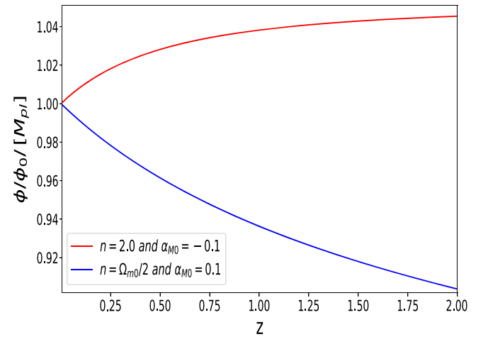
FIG. 5. Evolution of \phi/\phi(z=0) at late times. We have considered values of \alpha_{M0} and n within values compatible with the stability of the theory.
