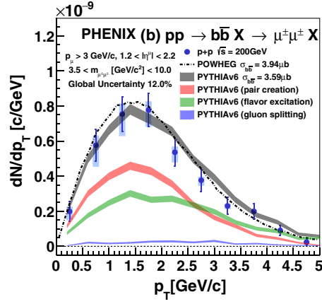
FIG. 26. The corrected \mu\mu yield as a function of pair p_T from (a) charm and (b) bottom decays. Presentation of the comparison to POWHEG and PYTHIA is the same as Fig. 25. The upper limits on panel (a) indicate 95% confidence level (For a data point with value d and statistical uncertainty \sigma , the upper limit u is determined by the following relation: \int_0^u f / \int_0^\infty f = 0.95 , where f is a Gaussian distribution with mean d and width \sigma ).
