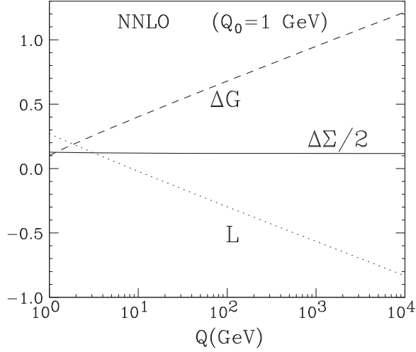
FIG. 3. Evolution of the quark and gluon spin contributions \frac{1}{2}\Delta\Sigma and \Delta G at NNLO, starting from the initial scale Q_0 = 1 GeV. We also show the evolution of \mathcal{L} following from Eq. (14).
