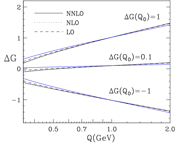
FIG. 4. Backward evolution of the gluon spin contribution \Delta G at LO (dashes), NLO (dots) and NNLO (solid line), starting from three different scenarios at the initial scale Q_0 = 1 GeV: \Delta G(Q_0) = +1, 0.1, -1 . The blue solid line corresponds to the leading 1/a_s term in Eq. (34).
