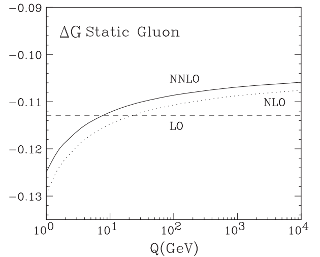
FIG. 5. Evolution of the ‘‘static’’ gluon solutions, starting from the initial scale Q_0 = 1 \text{ GeV} .
