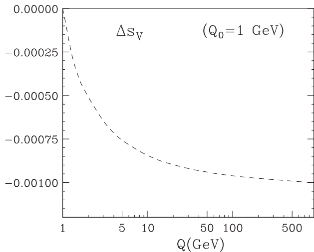
FIG. 6. Evolution of the perturbatively generated “valence” strange contribution \Delta s_V \equiv \Delta s - \Delta \bar{s} , starting from the initial scale Q_0 = 1 GeV.
