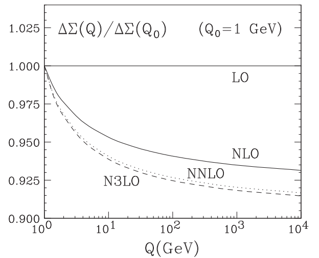
FIG. 1. Evolution of the first moment of the polarized singlet distributions at LO, NLO, NNLO and N 3 LO, starting from the initial scale Q_0 = 1 GeV.
