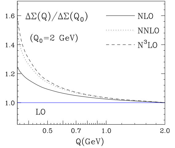
FIG. 2. Backward evolution of the first moment of the polarized singlet distributions at LO, NLO, NNLO, and N^3 LO, starting from the initial scale Q_0 = 2 GeV.
