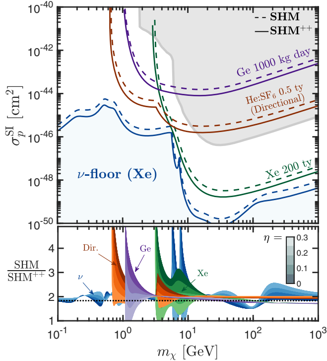
FIG. 5. Top: Using a set of toy experimental setups, we demonstrate the impact of the \text{SHM}^{++} on the sensitivity limits for three classes of detectors: a germanium experiment (purple), a directional He: \text{SF}_6 experiment (orange), and a xenon experiment (green). The lower blue-shaded region shows the neutrino floor for a xenon target while the gray-shaded region shows the already excluded parameter space (assuming the SHM). The dashed lines indicate the sensitivity assuming the SHM while the solid lines assume the \text{SHM}^{++} . For the \text{SHM}^{++} limits in the top panel, we have used the parameters from the lower half of Table I. Bottom: The ratio between the SHM and the \text{SHM}^{++} cross sections. The shading indicates the ratio for different values of \eta ( \eta = 0.2 corresponds to the ratio for the top panel). The black dotted line indicates the difference that arises solely from the different values of \rho_0 in the SHM and \text{SHM}^{++} ; deviations from this line arise from the different velocity distributions.
