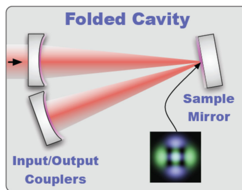
FIG. 1. A high-finesse cavity configuration, with a folding mirror (the sample to be measured) equidistant from the input and output mirrors. The inset image shows the TEM20 and TEM02 modes used to make the coating thermal noise measurement. Since these modes overlap only in a small central area, noise in the coating causes changes in the difference between their resonant frequencies, while most other noises sources cancel in this difference.
