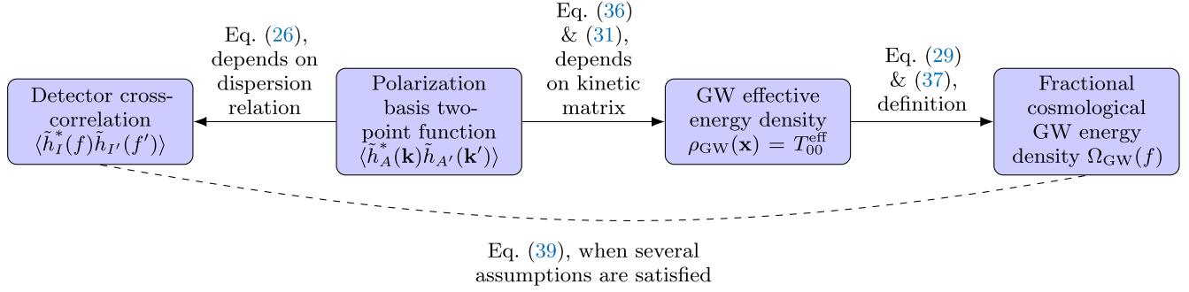
FIG. 1. Key quantities appearing in stochastic searches, and how they are related to each other. The relationships between them are theory dependent. The primary observable is the detector cross-correlation, but inferences are often stated in terms of the fractional cosmological GW energy density, or a parametrization thereof. Arrows point from more fundamental quantities to derived quantities.
