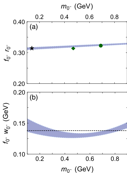
FIG. 2. (a) f_{0^-} r_{0^-} as a function of meson mass. It is nearly constant over a large range [80,82]. Black star—empirical value for the pion; green diamond—IQCD [34]; and green circle—IQCD [35]. (b) f_{0^-} w_{0^-} : w_{0^-} is the \langle 1/x \rangle -moment in Eq. (3). This function takes a minimum value in the neighbourhood of the s -quark current-mass and then evolves toward linear growth with m_{0^-} , up to logarithmic corrections. The dotted black line marks the mean value. The bands in both panels describe the range of results obtained for \omega \in [0.4, 0.6] \text{ GeV} .
