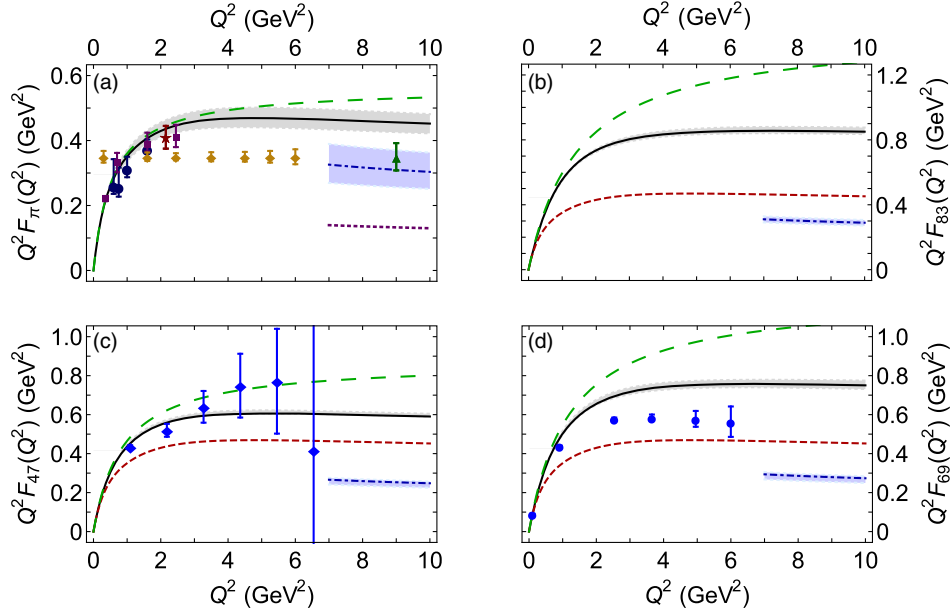
FIG. 1. Elastic form factors of pionlike pseudoscalar mesons. (a) physical pion, m_\pi = 0.14 GeV; (b) mass-degenerate quarks, meson mass = 0.83 GeV; (c) meson mass = 0.47 GeV; and (d) meson mass = 0.69 GeV. Curves in each panel. Solid black curve within grey bands—our prediction: obtained with w = 0.5 \pm 0.1 GeV in Eq. (8); long-dashed green curve—single-pole vector meson dominance result obtained with vector meson mass, m_V , computed consistent with the form factor prediction [see Eq. (15)]; and dot-dashed blue curve within blue bands—result from hard-scattering formula, Eq. (1), computed with the consistent meson decay constant and PDA. (a). Dotted purple curve—Eq. (1) computed with the consistent pion decay constant and asymptotic DA, \varphi_\infty(x) = 6x(1-x) ; filled-circles and -squares—data described in Ref. [15]; and filled gold diamonds and green triangle—projected reach and accuracy of forthcoming experiments [18,74]. For comparison, the dashed red curve in the other panels is the black curve from (a), viz. the physical-pion form factor prediction. (c) filled blue diamonds, IQCD results in Ref. [34]; and (d) filled blue circles, IQCD results in Ref. [35].
