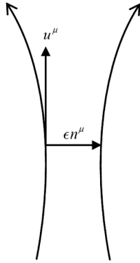
FIG. 1. Timelike geodesics for two nearby falling particles, with 4-velocity u^\mu , and separation s^\mu = \epsilon n^\mu , where n^\mu is a unit spacelike vector.
