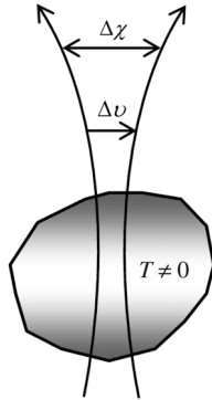
FIG. 2. Distance and velocity between two nearby timelike geodesics after interaction with the thermal bath of gravitons.
