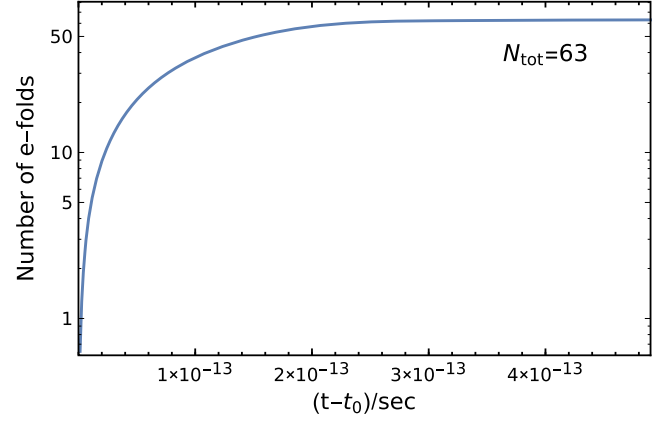
FIG. 3. Number of inflationary e-folds vs time for the 2-field model. Input parameters for Model A from the main text are used.
