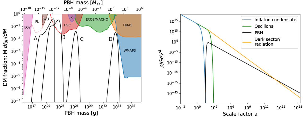
FIG. 2. (Left) DM fraction in primordial black holes. Fits for parameter choices corresponding to Model A, B, C and D are shown. Constraints from extragalactic \gamma -rays from BH evaporation [67] (EG \gamma ), femto-lensing [68] (FL), white dwarf abundance [69] (WD), Kepler star milli/micro-lensing [70] (K), Subaru HSC micro-lensing [61] (HSC) and MACHO/EROS/ OGLE micro-lensing [71] (ML) are displayed. Dashed FL line indicates that extended nature of the source as well as wave optics effects render GRB femtolensing constraints less effective [60]. Dashed line indicates that HSC constraints [72] are expected to be weaker than reported when PBH Schwarzschild radius becomes smaller than the wavelength of light [62,63]. (Right) Evolution of cosmological density for parameters of Model A. Contributions from the un-fragmented inflaton, oscillons, PBHs as well as the radiation sector are shown.
