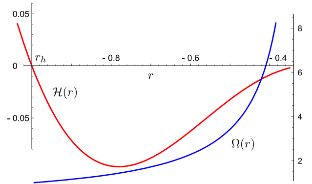
FIG. 1. The functions \mathcal{H}(r) and \Omega(r) for the Schwa-Bach black hole in the form (2.2). The first 20 terms in (5.3) for \mathcal{H} agree with a numerical solution with precision 10^{-4} , and the first 40 terms in (5.2) for \Omega agree with precision 10^{-5} on [-1, -0.5] . The horizon is at r_h = -1 , and k = 0.5 , b = 0.3633018769168 , which are the same values as in Ref. [6].
