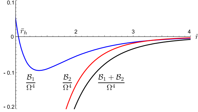
FIG. 3. The Bach tensor components (3.3), entering (6.1) and (6.2), as functions of \bar{r} . For the special value of b as in Fig. 1, they approach zero for large \bar{r} .
