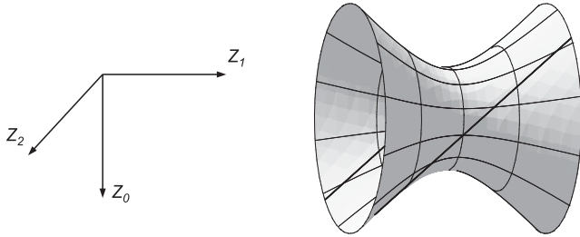
FIG. 1. The 2-hyperboloid visualizes the \text{dS}_2 factor \text{AdS}_2 factor of the LCBP universe (4) in the embedding coordinates (21). Each point corresponds to a 2-sphere of a constant radius b in the four-dimensional spacetime. The parallel solid lines Z_0 + Z_1 = 0 ( \Leftrightarrow Z_2 = \pm b ) are the histories of two of these spheres, propagating at the speed of light from one side of the universe to the other; cf., [8] for a similar discussion in the case of the solutions of [7].
