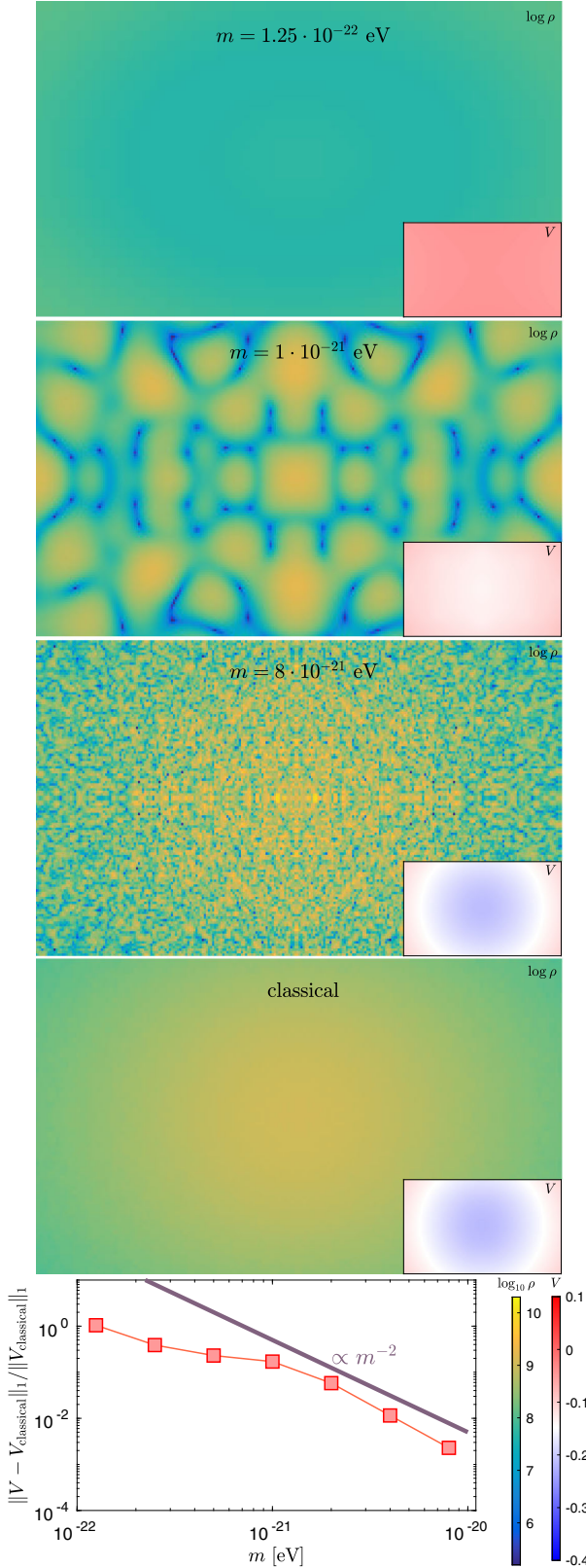
FIG. 6. Convergence of the 2D Gaussian collapse problem with warm initial conditions to the classical limit. Solution is zoomed in on [\frac{3}{8}, \frac{5}{8}] \times [\frac{7}{16}, \frac{9}{16}] . The potential converges to the classical limit as m^{-2} .
