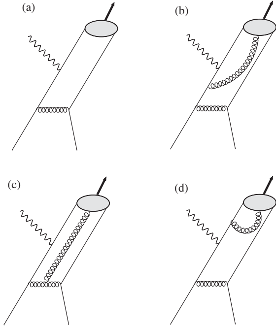
FIG. 2. Typical leading-order Feynman graphs for \gamma q \rightarrow \pi^0 q . (a) For a 2-particle Fock component of a pseudoscalar meson. (b), (c) Contribution from the q\bar{q}g Fock component without and with triple gluon coupling. (d) A soft contribution which is to be considered as part of the 3-particle DA.
