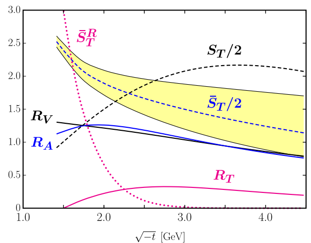
FIG. 1. The form factors for \pi^0 photoproduction scaled by t^2 . The dimension is GeV 4 . For the transversity form factor the value of the parameter A is 0.5 GeV -2 . The upper (lower) edge of the band for \tilde{S}_T is evaluated from A = 0.3(0.7) GeV -2 .
