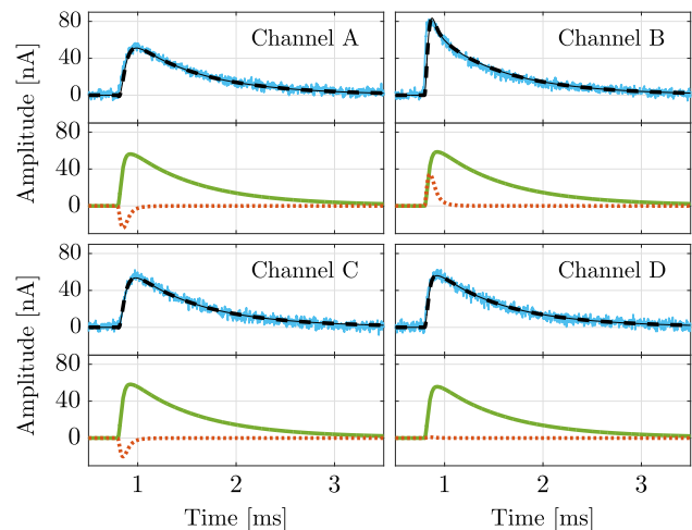
FIG. 7. Results of the 2T-fit algorithm for an example event chosen from the ^{71}\text{Ge} L -shell capture peak in Run 2. The traces and fits from all four phonon channels, labeled A–D (where channel A is the outer ring) are given. For each channel, the raw trace (blue solid) is compared to the final total fit (black dashed) which is a linear combination of the slow (green solid) and fast (orange dotted) templates. The channel with the largest fast-template amplitude, channel B for this event, is the channel of which the sensors are closest to the initial recoil.
