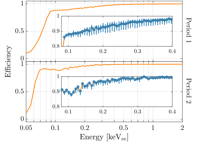
FIG. 16. Efficiency of the pulse-shape based cuts for Run 2 Period 1 (top) and Period 2 (bottom) as a function of electron-equivalent energy. Almost all loss in efficiency is due to the low-frequency noise cut, with the sharp drop in efficiency below 100 \text{ eV}_{\text{ee}} due to the kernel-density-estimate portion of that cut. The insets give an enlargement in the \mathcal{O}(100 \text{ eV}_{\text{ee}}) range, where the systematic uncertainty from varying the pulse shape, shown by the error bars, is largest. The average statistical uncertainty for each bin, due to the number of traces simulated, is 1.2%.
