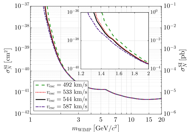
FIG. 29. Effect on the Run 2 best-fit limit from varying the Galactic escape velocity v_{\text{esc}} in the Maxwellian halo model while keeping all other parameters constant. Curves shown are the median values of the 2007 and 2014 RAVE survey results at 544 \text{ km s}^{-1} (black solid) and 533 \text{ km s}^{-1} (red dotted), respectively, as well as the 90% confidence bounds of the 2014 result at 492 \text{ km s}^{-1} (green dashed) and 587 \text{ km s}^{-1} (purple dot-dashed). The inset shows an enlargement below WIMP masses of 2 \text{ GeV}/c^2 . Varying v_{\text{esc}} changes the lowest WIMP mass that can produce recoils above threshold, while the impact on the limit at higher masses is negligible.
