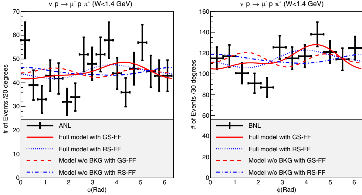
FIG. 14. ANL and BNL distribution of events in the pion azimuthal angle in the \pi N rest frame with W < 1.4 GeV for the \mu^- p \pi^+ final state. Curves are flux-averaged, area-normalized prediction of the model for d\sigma/d\phi .
