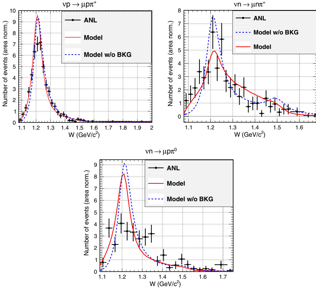
FIG. 11. W distribution for different neutrino CC channels from Ref. [25]. Curves are the model predictions with (solid red) and without (dashed blue) background.
