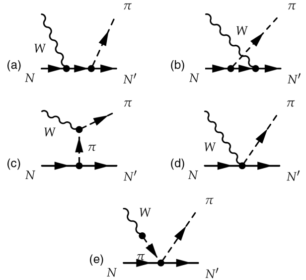
FIG. 3. Nonresonant pion production diagrams: (a) nucleon pole (NP), (b) crossed nucleon pole (CNP), (c) pion-in-flight (PIF), (d) contact term (CT), and (e) pion pole (PP).
