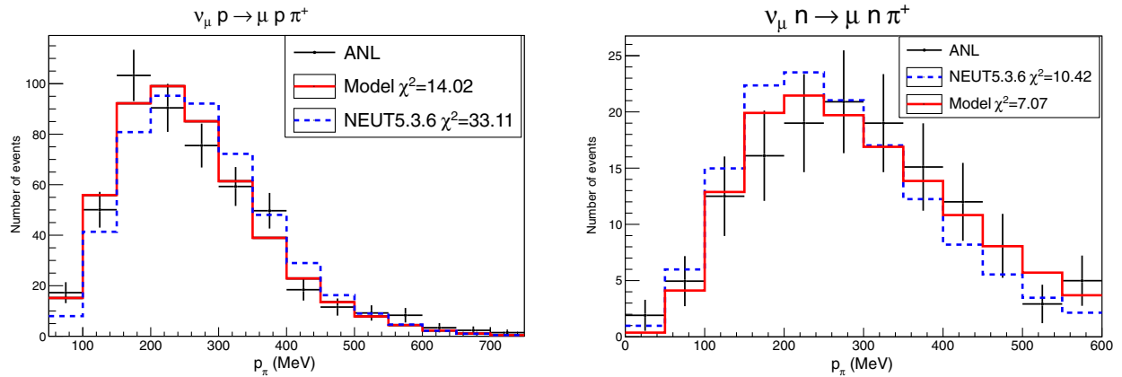
FIG. 9. Pion momentum distribution for the \nu p \rightarrow \mu p \pi^+ (left) and \nu n \rightarrow \mu n \pi^+ (right) channels from ANL [37]. Model (solid red) and RS model (dashed blue) predictions of flux-averaged p_\pi -differential cross sections (with W < 2 GeV cut), normalized to data, are also presented for the two channels.
