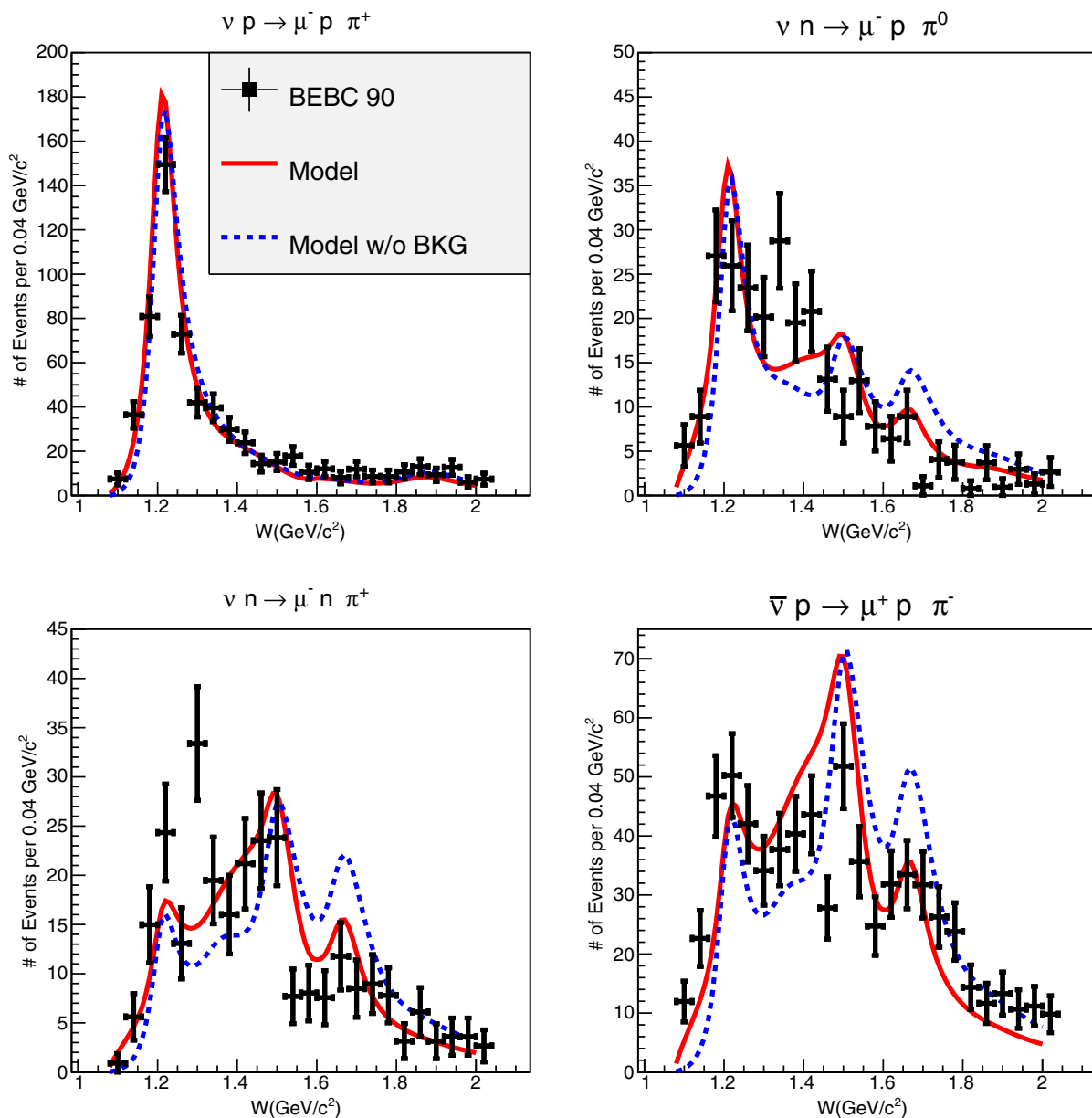
FIG. 10. W distribution for different neutrino and antineutrino CC channels from Ref. [30]. Curves are the model predictions with (solid red) and without (dashed blue) background.
