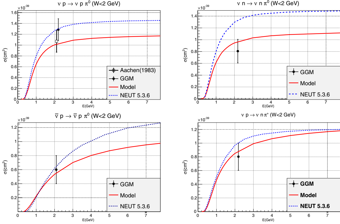
FIG. 8. Total cross section for NC (anti)neutrino channels. Data are from [39], and curves are model (solid red) and NEUT (dashed blue) predictions, with an invariant mass cut W < 2 GeV.
