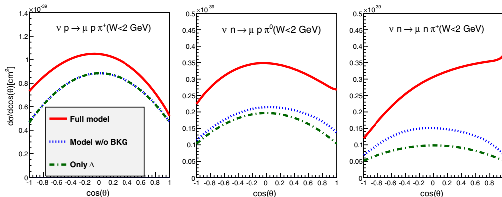
FIG. 13. The differential cross section averaged over T2K flux in terms of the polar angle. The dotted blue curve shows the model prediction for resonant interaction (up to W = 2 GeV), while the dashed green curve is only for the dominant \Delta resonance. The solid red curve shows the full model.
