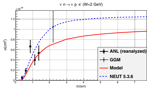
FIG. 7. Total cross section as a function of neutrino energy for the \nu n \rightarrow \nu p\pi^- channel. The model (solid red) and NEUT predictions (dashed blue) have an invariant mass cut W < 2 \text{ GeV} . Data are from [39].
