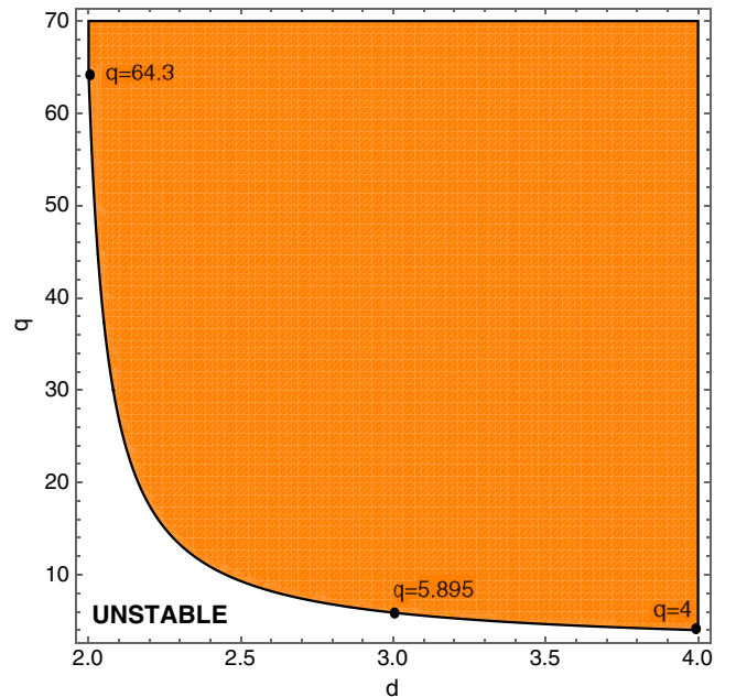
FIG. 2. Plot of q_{\text{crit}} as a function of d . The orange region corresponds to q > q_{\text{crit}} , where \Delta_{\phi^2} is real, and the theory is not obviously unstable. For integer dimensions, we obtained q_{\text{crit}}(2) \approx 64.3 , q_{\text{crit}}(3) \approx 5.9 , and q_{\text{crit}}(4) = 4 .
