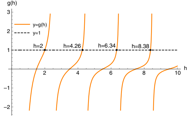
FIG. 1. The graphical solution of the eigenvalue equation g(h) = 1 in d = 1 . This method works for finding the real solutions only; it misses the complex solution h_0 = \frac{1}{2} + 1.525i .
