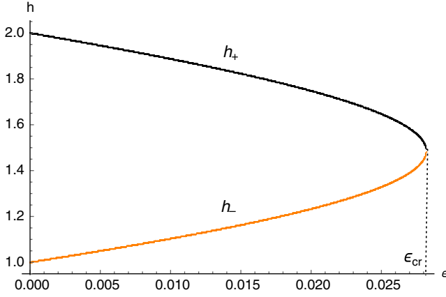
FIG. 3. Plot of the two lowest operator dimensions h_- and h_+ as a function of \epsilon . As \epsilon increases, h_- approaches h_+ , and at \epsilon_{\text{crit}} \approx 0.02819 , they merge and go off to the complex plane.
