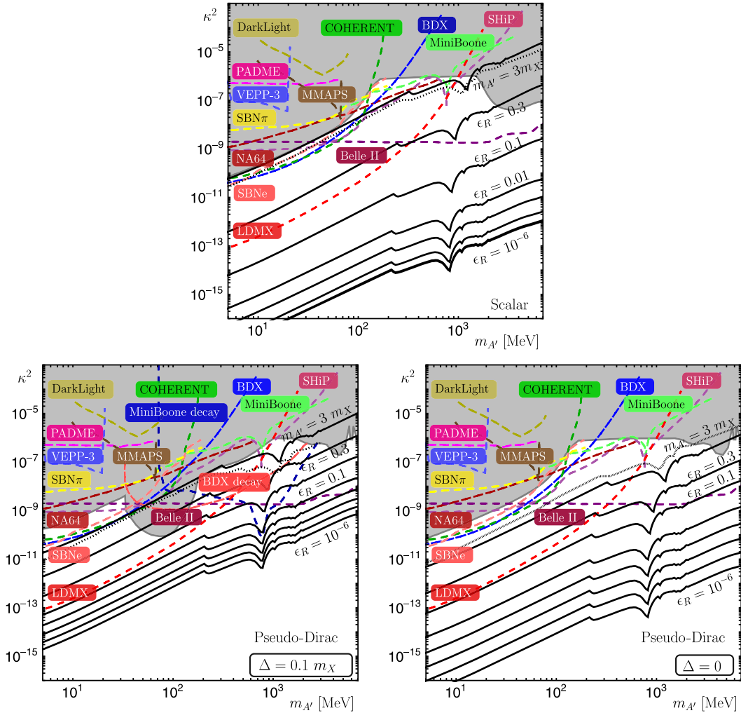
FIG. 1. Thermal targets and accelerator search experiments. Solid black contours: Thermal target contours in dark photon parameter space (m_{A'}, \kappa^2) for \alpha_X = 0.5 in the nondegenerate cases with m_{A'} = 3m_X and \epsilon_R \equiv (m_{A'}^2 - 4m_X^2)/(4m_X^2) = 0.3 , and in the degenerate cases with \epsilon_R = 10^{-n} , where n = 1, 2, \dots, 6 . In the scalar case (top) the thermal relic contours reach a floor near \epsilon_R = 10^{-6} , where the thermal relic abundance requirement becomes inconsistent with the requirement that the dark photon decay is dominantly invisible. The \epsilon_R = 10^{-5} contour is displayed in this plot, but is close enough to the \epsilon_R = 10^{-6} contour that they appear to overlap. In the pseudo-Dirac case (bottom) the thermal relic contours extend to arbitrarily low values of \kappa^2 with appropriate choice of \epsilon_R , but we display only a small number of contours to avoid clutter. In the bottom left panel, the mass splitting is \Delta = 0.1m_X , and these models evade direct detection bounds. In the bottom right panel, \Delta = 0 , which illustrates the effect of decreasing \Delta on the thermal target regions. Dotted black contours: Thermal target contours for m_{A'} = 3m_X from relativistic treatments of freeze-out for the scalar [33] and pseudo-Dirac [11] cases. Gray shaded: Regions excluded by current bounds (see text). Dashed contours: Projected reaches of proposed dark photon and dark matter accelerator searches (see text).
