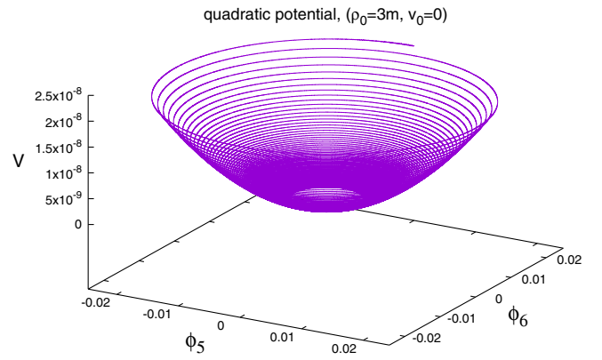
FIG. 2. Numerical solution of the equations of motion (16) and (17) in a quadratic potential with initial \rho_0 = 3m, v_0 = 0 , over a period of 2 \times 10^6 Planck times.
