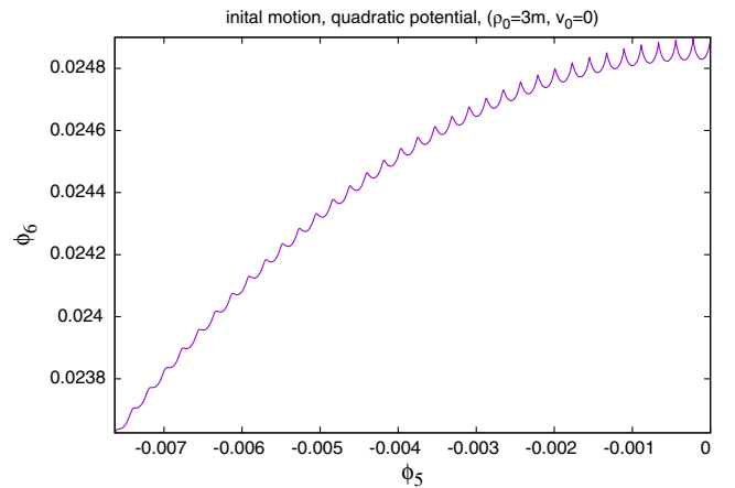
FIG. 3. The initial trajectory of the previous figure, projected into the \varphi_5 - \varphi_6 plane, which illustrates the initial transient behavior that dies out after roughly 2000 Planck times.
