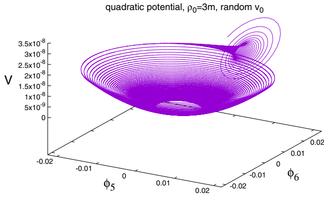
FIG. 4. Same as Fig. 2, but with a random initial velocity v_0 . The transient behavior is clearly seen in this example.
