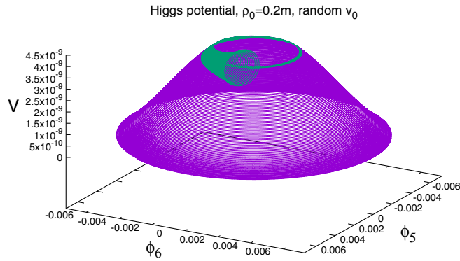
FIG. 6. Numerical solution of the equations of motion (16) and (17) in a Higgs potential with initial \rho_0 = 0.2m and random v_0 , over a period of 1 \times 10^6 Planck times. The initial transient behavior is shown in green.
