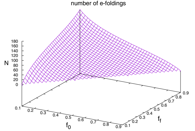
FIG. 8. The number of e -foldings N , in the Higgs potential case, as a function of the inflaton field \rho = |\varphi| at the start and end of inflation. The latter are displayed as fractions f_0 = \rho_{\text{initial}}/m and f_f = \rho_{\text{final}}/m of the minimum of the Higgs potential at \rho = m .
