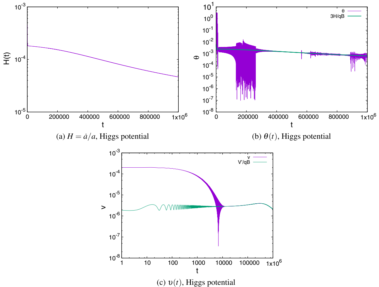
FIG. 7. For the example of the Higgs potential with a random initial v_0 : (a) The expansion rate H = \dot{a}/a . (b) Comparison of the computed \theta(t) in the \varphi_5 - \varphi_6 plane with the slow spiral prediction (24). (c) Comparison of the speed v(t) in the \varphi_5 - \varphi_6 plane with the slow spiral prediction (26).
