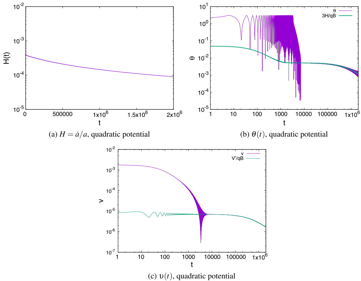
FIG. 5. For the example of the quadratic potential with a random initial v_0 : (a) The expansion rate H = \dot{a}/a . (b) Comparison of the computed \theta(t) in the \varphi_5 - \varphi_6 plane with the slow spiral prediction (24). (c) Comparison of the speed v(t) in the \varphi_5 - \varphi_6 plane with the slow spiral prediction (26).
