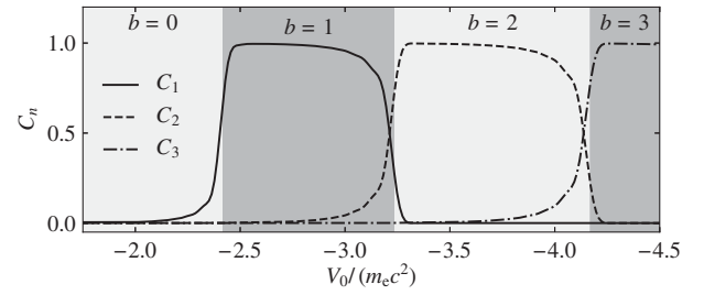
FIG. 3. n -pair probabilities C_n as a function of the maximal potential strength V_0 after the potential has been smoothly turned off with a total interaction time T = 93\hbar/(m_e c^2) . Other parameters are as in Fig. 2. The gray shaded areas indicate parameter regions with a particular number of supercritical quasibound states b .
