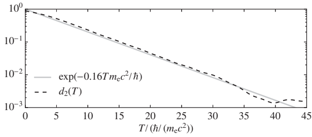
FIG. 4. Decay probability d_2 as a function of the interaction time T after the potential has been smoothly turned off (dashed black line) and an exponential fit to the data (solid gray line). The potential height is V_0 = -3.6m_e c^2 and other parameters are as in Fig. 1.
