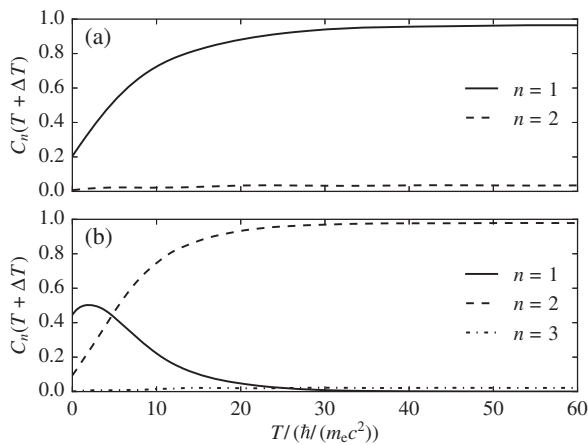
FIG. 2. n -pair probabilities C_n as a function of the interaction time T after the potential has been smoothly turned off with \Delta T = 4.7\hbar/(m_e c^2) for V_0 = -2.85m_e c^2 in (a) and V_0 = -3.6m_e c^2 in (b). Other parameters are as in Fig. 1.
