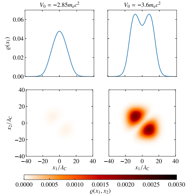
FIG. 5. Single- and two-pair spatial densities \rho(x_1) and \rho(x_1, x_2) as calculated for the parameters as in Fig. 2 and a total interaction time T = 90\hbar/(m_e c^2) . The left column corresponds to a potential strength of V_0 = -2.85m_e c^2 and the right one is for V_0 = -3.6m_e c^2 .
