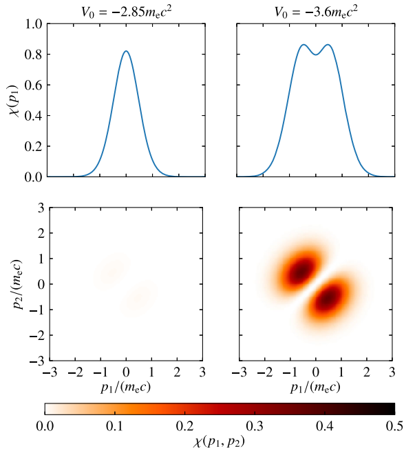
FIG. 6. Single- and two-pair momentum spectra \chi(p_1) and \chi(p_1, p_2) of the created electrons as calculated for the parameters as in Fig. 2 and a total interaction time T = 50\hbar/(m_e c^2) . The left column corresponds to a potential strength of V_0 = -2.85m_e c^2 and the right one is for V_0 = -3.6m_e c^2 .
