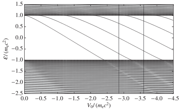
FIG. 1. Energy eigenvalues \mathcal{E} of the discretized one-dimensional Dirac Hamiltonian with the potential (32) with W = 0.3\lambda_C and D = 3.2\lambda_C as a function of the potential strength V_0 with \lambda_C denoting the Compton wavelength. Gray shaded areas indicate the continuous spectrum of the underlying Dirac Hamiltonian \hat{H}_D . For the discretization of the Dirac Hamiltonian a regular spatial grid running from -34.25\lambda_C to 34.25\lambda_C with 512 grid points was applied. The two vertical lines indicate the potential strengths that are employed in Figs. 2(a) and 2(b).
