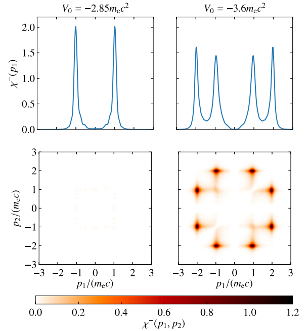
FIG. 7. Single- and two-pair momentum spectra \chi^-(p_1) and \chi^-(p_1, p_2) of the created positrons as calculated for the parameters as in Fig. 2 and a total interaction time T = 50\hbar/(m_e c^2) . The left column corresponds to a potential strength of V_0 = -2.85m_e c^2 and the right one is for V_0 = -3.6m_e c^2 .
