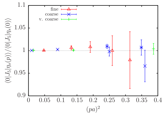
FIG. 5. The ratio of the matrix element between vacuum and \eta_s of the pseudoscalar density at nonzero spatial momentum to that at zero momentum, as a function of the square of the meson spatial momentum in lattice units. Symbols as for Fig. 4.
