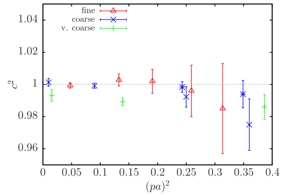
FIG. 4. The speed of light, defined in the text, determined from our \eta_s meson energies as a function of the square of their spatial momentum in lattice units. Note the expanded y-axis scale. Results from very coarse set 1 are given by green pluses, coarse set 2 by blue crosses and set 3 by blue bursts, and fine set 4 by red triangles.
