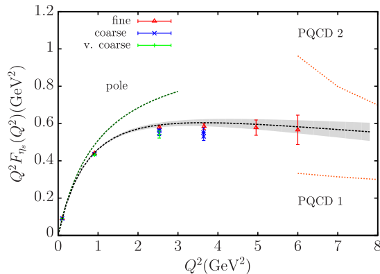
FIG. 2. Lattice QCD results for the vector form factor of the \eta_s meson, multiplied by Q^2 to focus on the large Q^2 behavior, plotted as a function of Q^2 . From coarse to fine: set 1 results are given by green pluses, set 2 by blue crosses, set 3 by blue bursts and set 4 by red triangles. Error bars include statistical/fit errors and uncertainties from the lattice spacing correlated between points. The black dashed line and grey band (for \pm 1\sigma ) give the physical-point curve discussed in the text. The green dashed line marked “pole” gives the pole form ( P_\phi^{-1} ), for comparison. The orange dotted line marked “PQCD 1” gives the asymptotic perturbative QCD prediction and that marked “PQCD 2” includes nonasymptotic corrections to the distribution amplitude discussed in the text.
