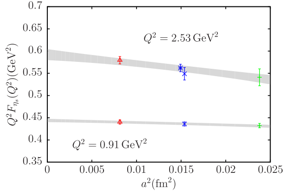
FIG. 6. We show here two slices through Fig. 2 at two different values of Q^2 , 2.53 \text{ GeV}^2 and 0.91 \text{ GeV}^2 , plotted against the square of the lattice spacing. The points (symbols as for Fig. 4) show results at appropriate nearby values of Q^2 (see Table II) and include correlated uncertainties from the lattice spacing. The grey bands show our fit result using Eq. (5), now as a function of a^2 but with \delta m set to zero.
