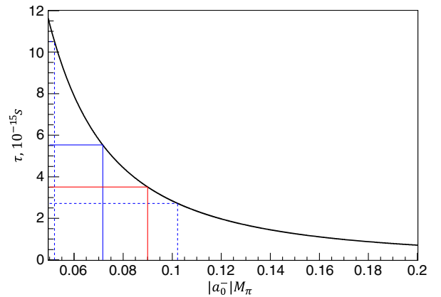
FIG. 17. Ground state A_{\pi K} lifetime \tau_{1S} versus a_0^- from the Q analysis. Experimental results (blue lines) are compared to the theoretical prediction (red lines).
