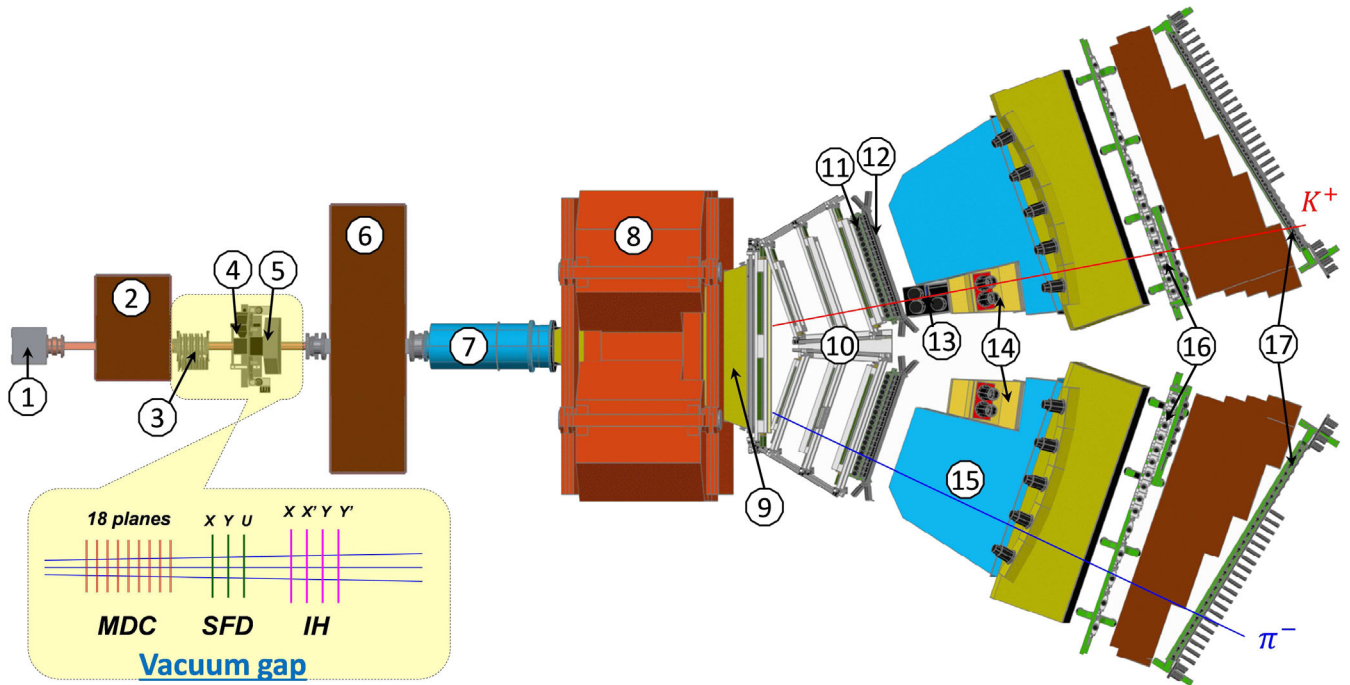
FIG. 3. General view of the DIRAC setup [1: target station; 2: first shielding; 3: micro drift chambers (MDC); 4: scintillating fiber detector (SFD); 5: ionization hodoscope (IH); 6: second shielding; 7: vacuum tube; 8: spectrometer magnet; 9: vacuum chamber; 10: drift chambers (DC); 11: vertical hodoscope (VH); 12: horizontal hodoscope (HH); 13: aerogel Cherenkov (ChA); 14: heavy gas Cherenkov (ChF); 15: nitrogen Cherenkov (ChN); 16: preshower (PSh); 17: muon detector (Mu)].
