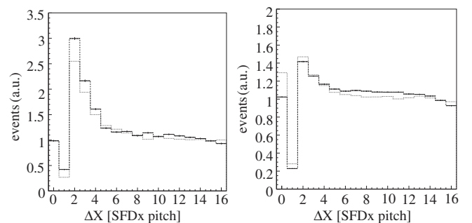
FIG. 12. Distributions over distance between tracks measured by SFDx plane in units of the detector pitch (column number). Left: \Delta n_X distribution in SFDx for track pairs with small distance in Y plane ( \Delta n_Y < 3 ). Right: \Delta n_X distribution in SFDx without any constraint in Y plane. Solid line: experimental data; dotted line: MC data (see text).
