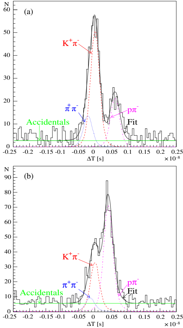
FIG. 9. (a) Difference of particle generation times for events with positively charged particle momenta ( 4.4 \div 4.5 ) GeV/c. Experimental data (histogram) are fitted by the event sum (black, solid): K^+\pi^- (red, dashed), \pi^+\pi^- (blue, dotted), p\pi^- (magenta, dotted-dashed) and accidentals (green, constant). (b) Similar distributions for events with positively charged particle momenta ( 5.4 \div 5.5 ) GeV/c.
