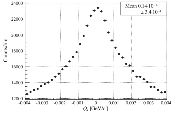
FIG. 7. Q_L distribution of \pi^+\pi^- experimental data with cut Q_T < 4 MeV/c (RUN2 to RUN4).
