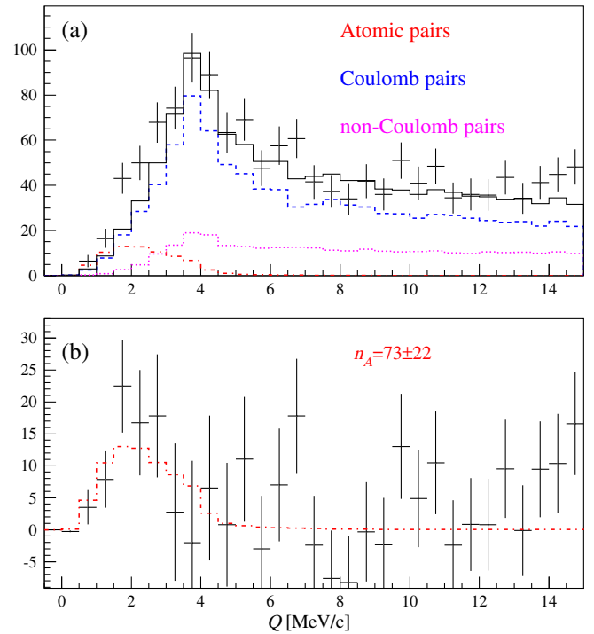
FIG. 14. (a) Experimental distribution of \pi^- K^+ and \pi^+ K^- pairs (points with error bars) for the platinum (Pt) target fitted by a sum of simulated distributions of “atomic,” “Coulomb” and “non-Coulomb” pairs. The background distribution of free (Coulomb and non-Coulomb) pairs is shown as black line; (b) difference distribution between the experimental and simulated free pair distributions compared with the simulated distribution of “atomic pairs.”
