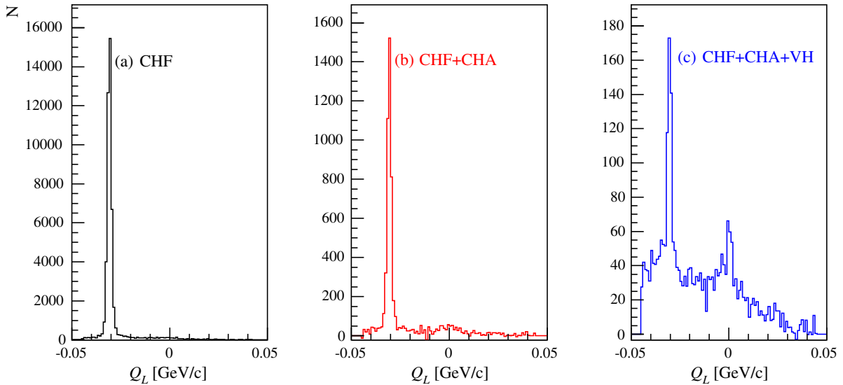
FIG. 10. Q_L distribution of \pi^- K^+ pairs after applying different criteria. (a) Distribution of potential \pi^- K^+ pairs requiring a ChF signal and Q_T < 4\text{MeV}/c , the dominant peak on the left side is due to miss identified p\pi^- pairs from \Lambda decay; (b) After adding request of ChA signal this peak is decreased significantly; (c) Additional criterion on TOFs between target and VH suppress background of p\pi^- and \pi^+\pi^- pairs substantially. The well-defined peak at Q_L = 0 is the \pi^- K^+ Coulomb peak.
