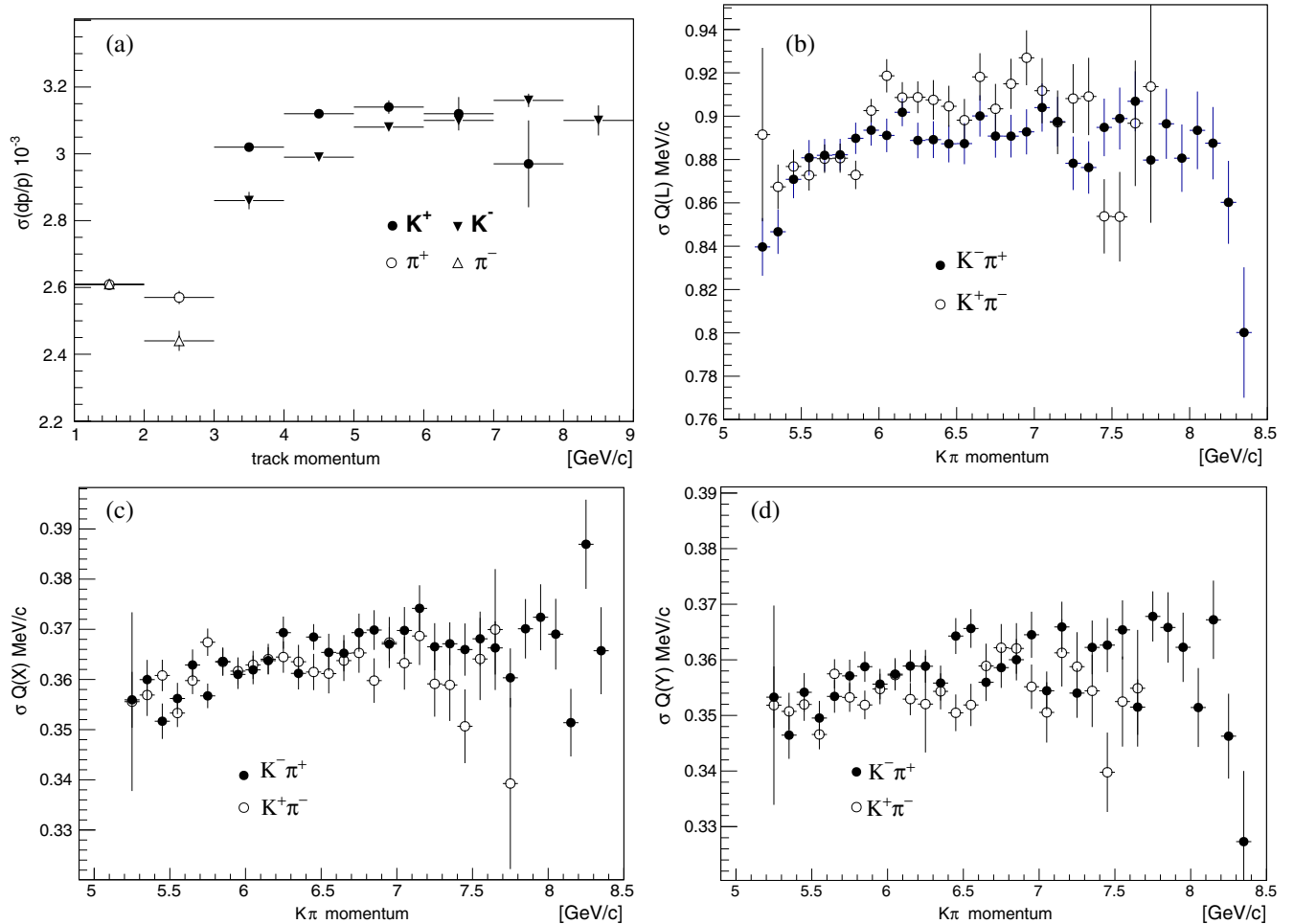
FIG. 13. Momentum resolution (a) as a function of the laboratory particle momentum and resolution of the relative momentum components Q_L (b), Q_X (c) and Q_Y (d) as a function of the total laboratory momentum of K^- \pi^+ (black) and K^+ \pi^- (white).
