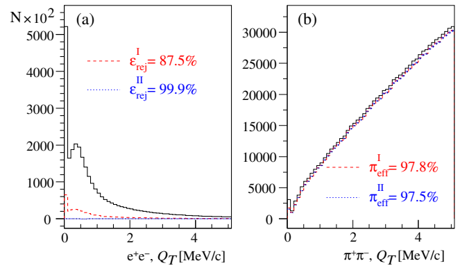
FIG. 8. Q_T distributions for (a) e^+e^- and (b) \pi^+\pi^- pairs without PSh amplitude criterion (black solid line), after amplitude criterion (red dashed line) and after additional subtraction of electron admixture in the accepted events (blue dotted line).
