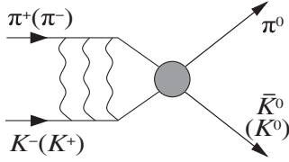
FIG. 1. The dominant decay channel of the \pi K atom. The wavy lines indicate Coulomb photons.
