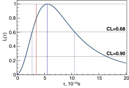
FIG. 16. Likelihood functions L(\tau) for Q analyses with Q_T < 4 MeV/c. The likelihood functions on the basis of both statistical and systematic errors (dashed green line) and on the basis of only statistical error (solid blue line) are presented. The vertical blue lines indicate the best estimate for \tau_{\text{tot}} and the corresponding confidence interval. The vertical red line is the theoretical prediction (2).
