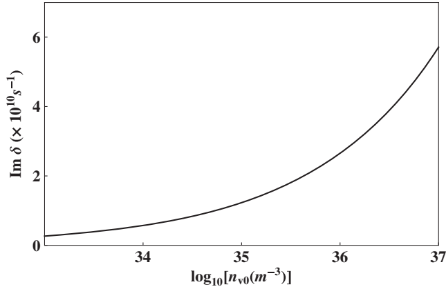
FIG. 3. Instability growth rate from Eq. (35) for \mathcal{E}_{\nu 0} = 10 MeV, v_T/c = 1/10 , n_0 = 10^{34} m ^{-3} , as a function of neutrino beam number density n_{\nu 0} , for \mathbf{k} \parallel \boldsymbol{\omega}_c .
