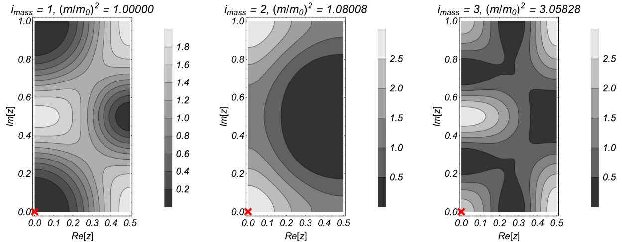
FIG. 2. The probability densities |\phi^{i_{\text{mass}}}(z)|^2 of the KK wave functions with mass eigenvalues that are unaffected ( i_{\text{mass}} = 1 )/perturbed ( i_{\text{mass}} = 2, 3 ) by the brane-localized mass at z = z_1 for M = 3 and h = 0.5 . A red cross denotes a position with the brane-localized mass. The corresponding mass eigenvalues after the perturbation are also shown. The values of the ratio (m/m_0)^2 before the perturbation are 1, 1, and 3, respectively.
