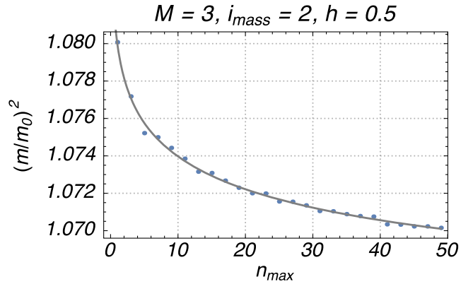
FIG. 4. The cutoff scale dependence of the squared mass ratio (m/m_0)^2 for a perturbed mode. Fitting parameters are chosen as (\alpha_1, \alpha_2, \alpha_3) = (1.07999, -0.00265445, 9.10443 \times 10^{-6}) . Note that the ratio before the perturbation is (m/m_0)^2 = 1 .
