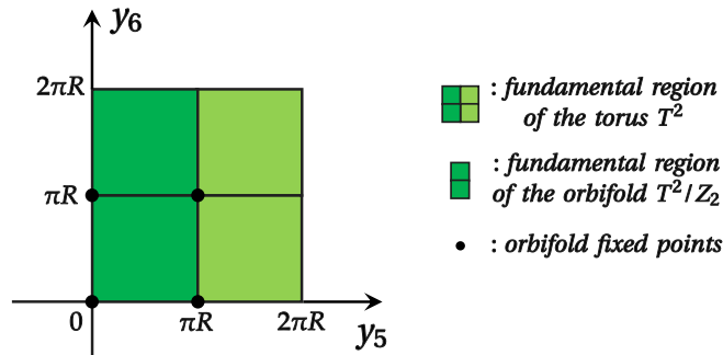
FIG. 1. The fundamental region of the orbifold T^2/Z_2 and the four fixed points on it.
