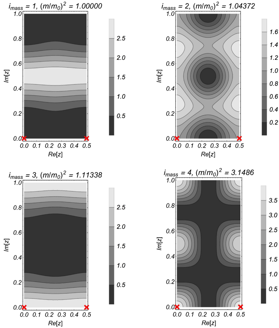
FIG. 3. The probability densities |\phi^{i_{\text{mass}}}(z)|^2 of the KK wave functions with mass eigenvalues that are unaffected ( i_{\text{mass}} = 1 )/perturbed ( i_{\text{mass}} = 2, 3, 4 ) by the brane-localized mass terms at z = z_1 and z = z_2 for M = 4 and h = 0.5 . The two red crosses in each panel denote the positions where the brane-localized mass terms are located. The corresponding mass eigenvalues after the perturbation are also shown. The values of the ratio (m/m_0)^2 before the perturbation are 1, 1, 1, and 3, respectively.
