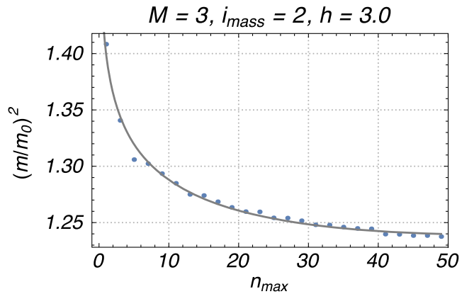
FIG. 5. The cutoff scale dependence of the squared mass ratio (m/m_0)^2 for a perturbed mode. Fitting parameters are chosen as (\alpha_1, \alpha_2, \alpha_3) = (1.39949, -0.0523681, 0.0009029) . Note that the ratio before the perturbation is (m/m_0)^2 = 1 .
