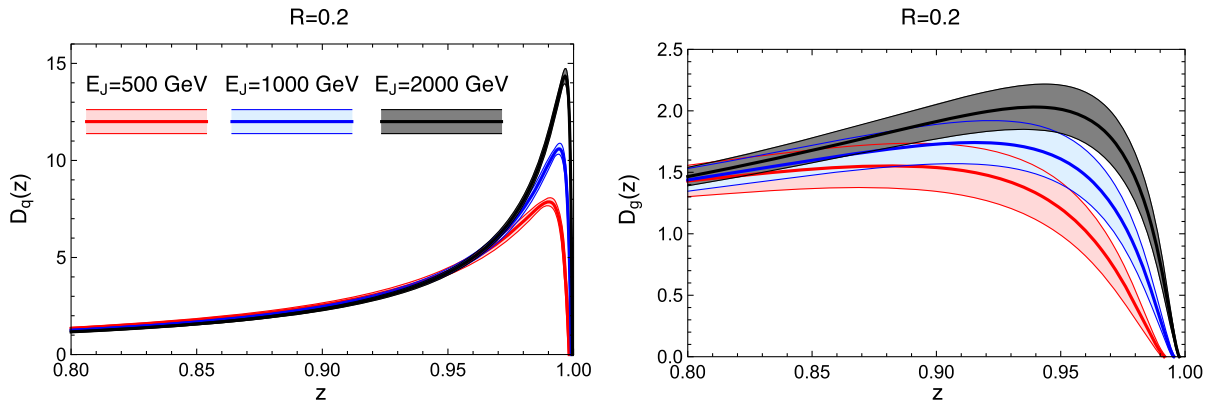
FIG. 2. D_{J_{q/q}}(z) (left panel) and D_{J_{g/g}}(z) (right panel) with different jet energies. Red, blue, and black curves correspond to jet energy E_J equal to 500, 1000, and 2000 GeV, respectively. The jet radius is chosen to be R = 0.2 and the factorization scale is \mu_f = E_J . Error estimation is described in the text.
