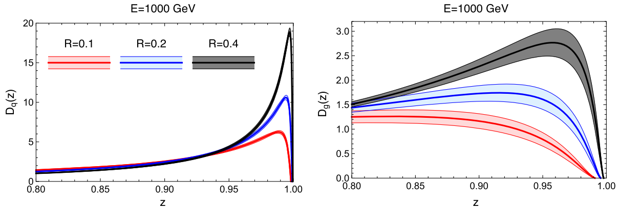
FIG. 3. D_{J_q/q}(z) (left panel) and D_{J_g/g}(z) (right panel) with different jet radii. Red, blue, and black curves correspond to the jet radius R equal to 0.1, 0.2, and 0.4, respectively. The jet energy is E_J = 1000 GeV and the factorization scale is \mu_f = E_J .
