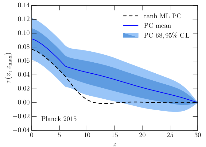
FIG. 6. Cumulative optical depth \tau(z, z_{\max}) in the Planck 2015 analysis. 68% and 95% CL constraints from the complete PC analysis compared with the chain ML tanh model also constructed from PCs (dashed line). PC analysis shows that the data prefer finite high redshift optical depth out to z \gtrsim 16 at 95% CL. The tanh model has essentially no optical depth for z \gtrsim 10 due to its steplike form. Both model classes have the same ionization history for z < 6 .
