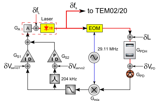
FIG. 5. Block diagram of control loops for the TEM00 mode. All of the important noise sources are indicated as \delta_i , and each loop component with nonzero gain value is marked with G_i . The TEM00 mode is locked to the cavity length using PDH in reflection. An additional 204 kHz loop is used to reduce frequency noise related to the locking scheme of TEM20/02 modes. More detail in text.
