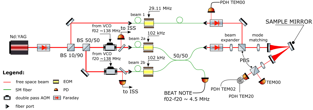
FIG. 3. The experimental setup for the multimode measurement involves a Nd:YAG laser (far left) and an in-vacuum high-finesse cavity (far right). In order to avoid multiple lasers, and the multiple sources of frequency and intensity noise they would introduce, a single laser beam is split into three paths, two of which are shifted in frequency (with AOMs), and each of which is independently phase modulated at its own radio frequency (with EOMs). The laser frequency is controlled to lock the TEM00 mode to the cavity length while the TEM02 and TEM20 modes are locked to the cavity by controlling their frequency differences with respect to the laser frequency. The primary output of the experiment is the difference between the TEM02 and TEM20 resonant frequencies (labeled BEAT NOTE), changes in which are dominated by the coating thermal noise of the sample.
