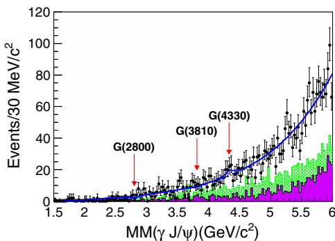
FIG. 13. The \gamma J/\psi recoil mass spectrum for \Upsilon(2S) \rightarrow \gamma \chi_{b1} \rightarrow \gamma J/\psi + \text{anything} in the \Upsilon(2S) data sample. The solid curve shows the result of the fit described in the text, including the G(2800) , G(3810) , and G(4330) states, with a common width fixed to 0.15 GeV and with central values indicated by the arrows. The dashed curve shows the fitted background. The shaded histogram is from the normalized J/\psi mass sideband events, and the cross-hatched histogram shows the normalized continuum contributions.
