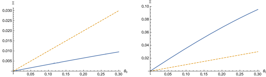
FIG. 6. Left: Thick curve, the rhs of Eq. (7.13), \Xi , for m/T = 0.1 and the maximal time of interaction \tau = 30 ; dashed curve, \dot{\theta}/T as functions of \theta_0 ; see Eq. (8.5). Right: The same as the maximal time of integration \tau = 3 .
