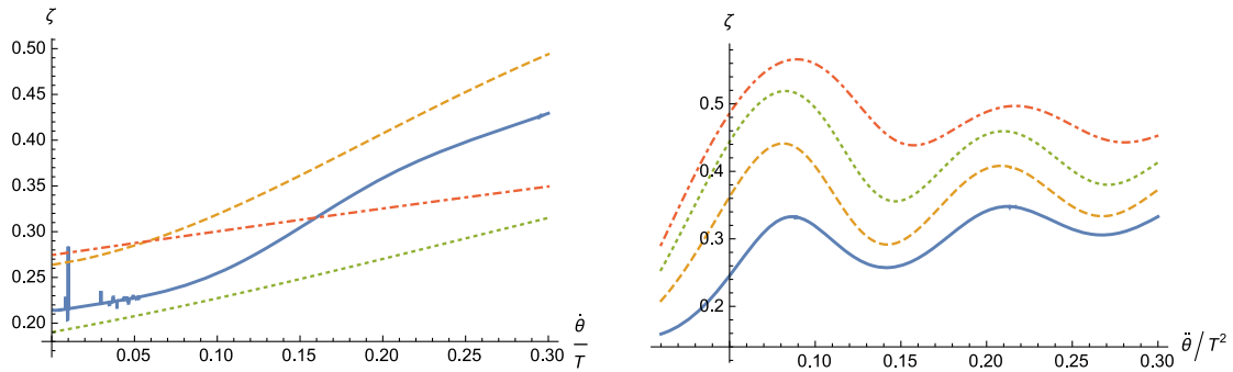
FIG. 4. Left: The relative difference, \zeta = \Xi/(\dot{\theta}/T) - 1 , as a function of \dot{\theta}/T for the cutoff of the time integration \tau = 30 (thick), 10 (dashed), 5 (dotted), and 3 (dot dashed) for fixed \ddot{\theta}/T^2 = 0.1 . Right: The same difference as a function of \ddot{\theta}/T^2 for fixed time of integration \tau = 10 and different \dot{\theta}/T = 0.1 (thick), 0.2 (dashed), 0.3 (dotted), and 0.4 (dot dashed).
