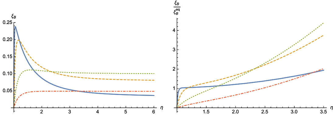
FIG. 1. Left: Evolution of \xi_B(\eta) according to Eq. (5.8) where C_B T_{in}^2 / (5f^2) = 0.1 for K = N = 20 (thick), 5 (dashed), 1 (dotted), and 0.3 (dot dashed). Right: Ratio of \xi_B(\eta) to its equilibrium value, \xi_B^{eq}(\eta) , determined by (5.9) for the same values of the parameters.
