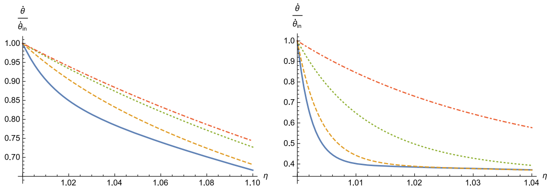
FIG. 2. Left: Evolution of \dot{\theta}(\eta) , normalized to its initial value, \dot{\theta}_{in} , for C_B T_{in}^2 / (5f^2) = 0.1 and K = N = 20 (thick), 5 (dashed), 1 (dotted), and 0.3 (dot dashed). Right: The same with C_B T_{in}^2 / (5f^2) = 1 and K = N = 50 (thick), 30 (dashed), 10 (dotted), and 3 (dot dashed).
