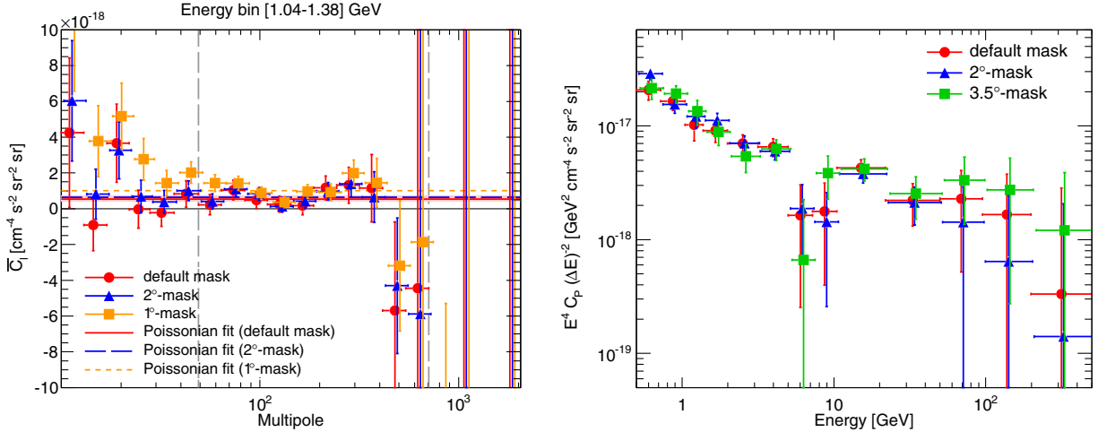
FIG. 17. Left: Comparison of the auto-APS in the energy bin from 1.04 to 1.38 GeV among the case with the default mask covering the sources in 3FGL (red circles), the case with the 2^\circ mask (blue triangles) and the one with the 1^\circ mask (orange squares). The solid red line marks the best-fit C_P for the default mask, with the pink band indicating its 68% C.L. error. The long-dashed blue line gives the best-fit C_P when the 2^\circ mask is employed and the short-dashed orange one for the case with the 1^\circ mask. The vertical gray dashed lines mark the signal region between \ell = 49 and 706. Right: Poissonian auto-APS as a function of energy for the case with the default mask (red circles), the 2^\circ mask (blue triangles) and the 3.5^\circ mask (green squares).
