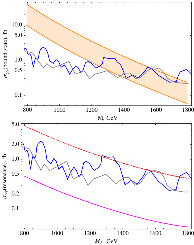
FIG. 2. Top panel: Diphoton signals from \bar{\Psi}\Psi , QCD bound states of VLQs, at \sqrt{s} = 13 TeV as a function of the lowest bound state mass M for the representation (3, 1, 5/3) . The signal strength is computed from the Coulomb potential calculations in Ref. [14]. The lower curve of the orange band corresponds to choosing N = 1 , while the top curve corresponds to N = 2 . Bottom panel: Diphoton resonant cross section at 13 TeV from production through a loop of VLQ in the representation (3, 1, 5/3) with mass 1 TeV, as a function of the resonance mass, for \lambda = 0.3 (magenta, solid line) and \lambda = 1 (red, dashed line). The gray (blue) curve in both panels is the current diphoton cross section limit from ATLAS (CMS).
