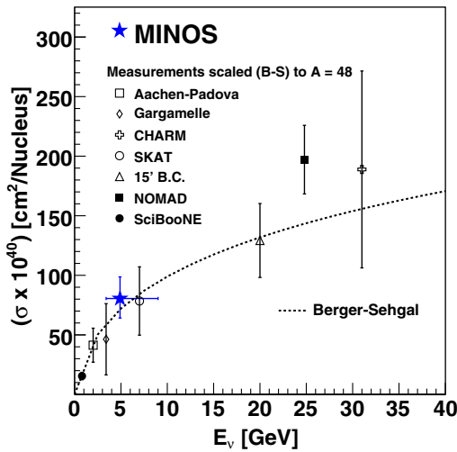
FIG. 12. Comparison of the MINOS \text{NC}(\pi^0) coherent-scattering total cross section (flux-averaged) to measurements obtained with \langle E_\nu \rangle at lower and higher values. Previous measurements are shown scaled to the MINOS target medium, \langle \mathcal{A} \rangle = 48 , for the purpose of comparison. Table I compares the previous measurements as reported, to the direct Berger-Sehgal prediction.
