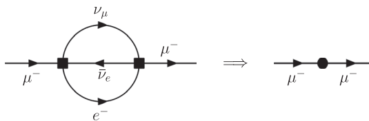
FIG. 2. In the amplitude for \mu^- \rightarrow \nu_\mu e^- \bar{\nu}_e \rightarrow \mu^- , the high-momentum intermediate-state particles are created and annihilated in a localized region. Their effects can therefore be reproduced by local operators.
