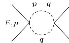
FIG. 6. Diagram of order g^2 for \psi\psi \rightarrow \psi\psi through an intermediate state with two \phi particles.
