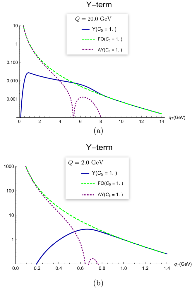
FIG. 3. The Y term (blue solid curves) calculated using the method of Eq. (57) and Sec. VIII. One calculation (a) is for a large scale, Q = 20.0 GeV and one calculation (b) is for a small scale, Q = 2.0 GeV. For comparison, the \text{FO}(q_T, Q) (green dashed) and \text{AY}_{\text{New}}(q_T, Q; \eta, C_5) (magenta dot-dashed) calculations are also shown. In all cases, C_5 = 1.0 . The curves are normalized to the value of \text{FO}(q_T, Q) at q_T = 1.0 GeV. In all cases, we take x = 0.1 and z = 0.5 .
