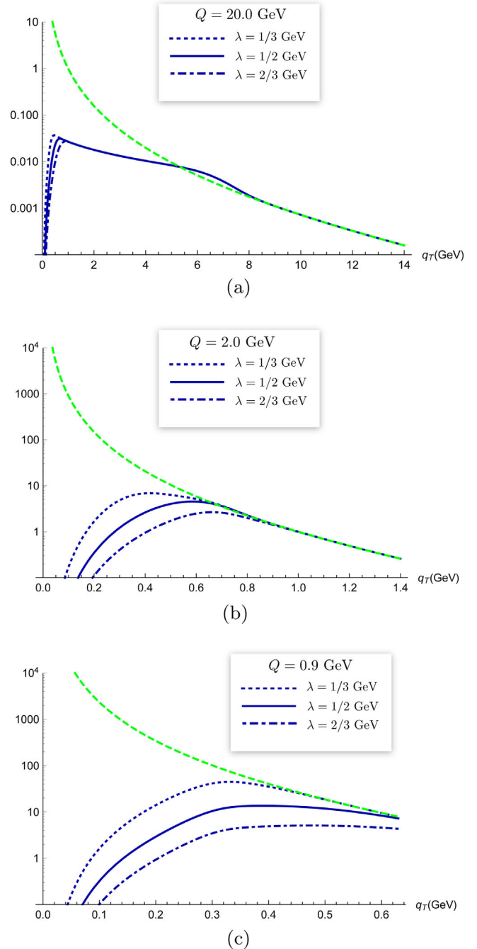
FIG. 4. The Y term calculated with C_5 = 1.0 and with the three values: \lambda = 1/3 GeV (blue dotted curves), \lambda = 1/2 GeV (blue solid curves) and \lambda = 2/3 GeV (blue dot-dashed curves). The green dashed curves show the fixed-order calculations. Graph (a) is for Q = 20 GeV, graph (b) is for Q = 2 GeV, and graph (c) is for Q = 0.9 GeV. (See text for further explanation.) In all cases, we take x = 0.1 and z = 0.5 .
