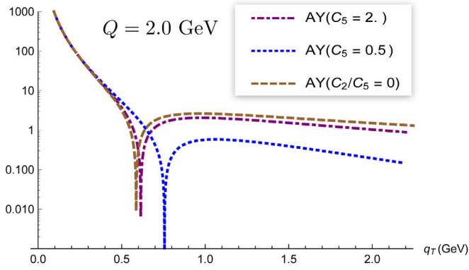
FIG. 2. The absolute value of the asymptotic term calculation with \Xi replaced by 1, and with the substitutions in Eqs. (65) and (66) and various choices for C_5 . The brown dashed curve is the limit of the standard CSS Y term approach. In all cases, C_2 = 1 . The blue dotted and magenta dash-dotted curves correspond C_5 = 0.5 and C_5 = 2.0 , respectively. All curves are normalized to \text{FO}(q_T, Q) for C_2/C_5 = 0 and q_T = 1 GeV. The variation between the curves can be viewed as an measure of the sensitivity of the \text{AY}(q_T, Q) calculation to different choices of C_5 . In all cases, we take x = 0.1 and z = 0.5 .
