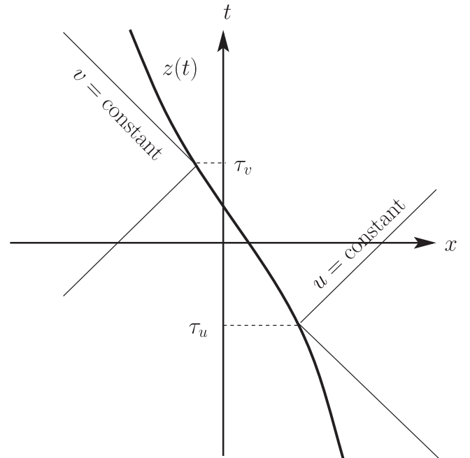
FIG. 1. The mirror moving along the trajectory z(t) divides the spacetime into two distinct regions to the right and the left of the mirror. Note that \tau_u and \tau_v denote the times when the incoming waves are reflected by the mirror and converted into outgoing waves to the right and the left of the mirror, respectively.
