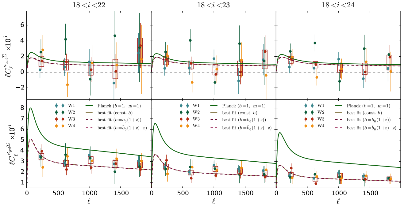
FIG. 2. Angular cross-power spectra of (1) \kappa_{\text{cmb}} and \Sigma (upper panels) and (2) \kappa_{\text{gal}} and \Sigma (lower panels) for three galaxy samples ( 18 < i < 22 , 18 < i < 23 , and 18 < i < 24 ). Data points are for individual CFHTLenS fields, and errors are estimated using 100 simulated \kappa_{\text{cmb}} maps and 100 randomly rotated \kappa_{\text{gal}} maps. The boxes represent the inverse-variance weighted sum of the four fields. The thick-solid, thin-solid, thick-dashed, and thin-dashed curves are the fiducial theoretical model using Planck 2015 parameters ( b, m = 1 ), the best-fit model assuming a constant b , the best-fit model assuming b(z) = b_0(1+z) , and the best-fit model assuming b(z) = \tilde{b}_0(1+z) - z , respectively. The three best-fit models use the combined constraints on b and m from jointly fitting the C_\ell^{\kappa_{\text{cmb}} \Sigma} and C_\ell^{\kappa_{\text{gal}} \Sigma} data.
