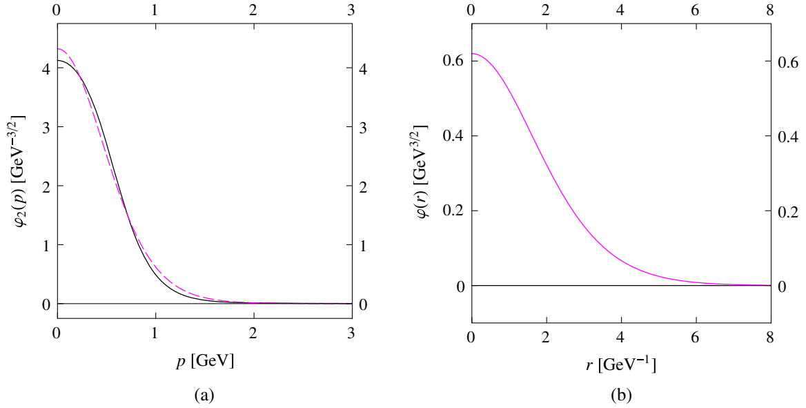
FIG. 3. Normalized radial independent Salpeter component defining, at least for Salpeter equations (2) characterized by the Lorentz structure 2\Gamma \otimes \Gamma = \gamma_\mu \otimes \gamma^\mu + \gamma_5 \otimes \gamma_5 - 1 \otimes 1 of their interaction kernels, the Salpeter amplitude (3) of any spin-singlet state, and thus, in particular, of any pseudoscalar meson. In momentum-space representation (a) we show its exact shape computed, via the relationship (7), from the quark mass function of Fig. 1 (black solid line) as well as an approximation deduced from a fit to the simplified functional dependence (10) (magenta dashed line); in configuration-space representation (b) we only depict the behavior of the Fourier-Bessel transform of the latter approximation (magenta solid line).
