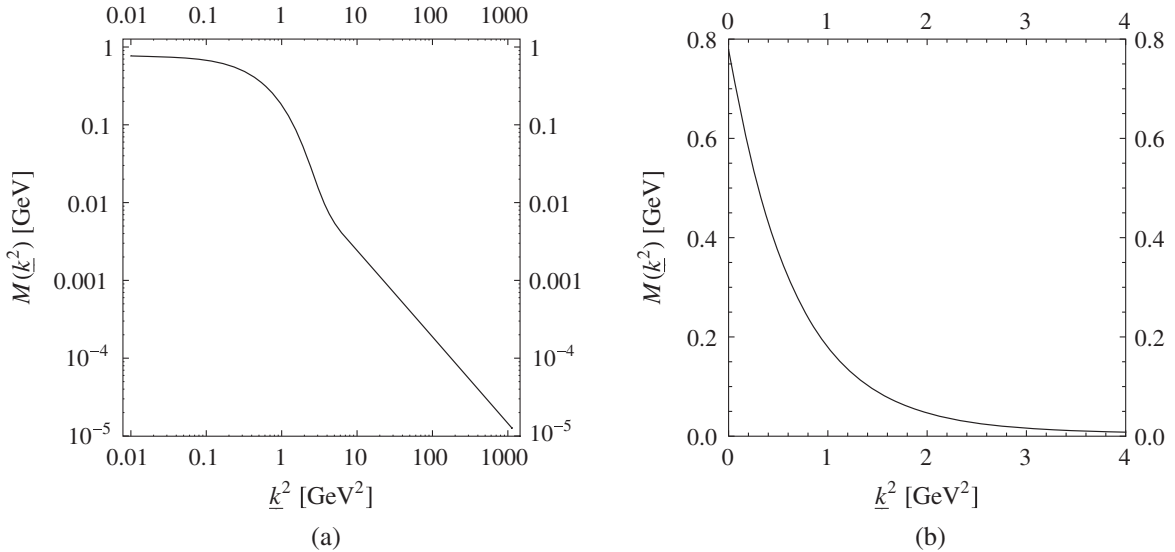
FIG. 1. Mass function M(\underline{k}^2) , derived by solution of the renormalization-group-improved rainbow-ladder approximation to the Dyson-Schwinger equation for the quark propagator, S(\underline{k}) , in the chiral limit (Fig. 2 of Ref. [13]), for double-logarithmic (a) and linear (b) scales.
