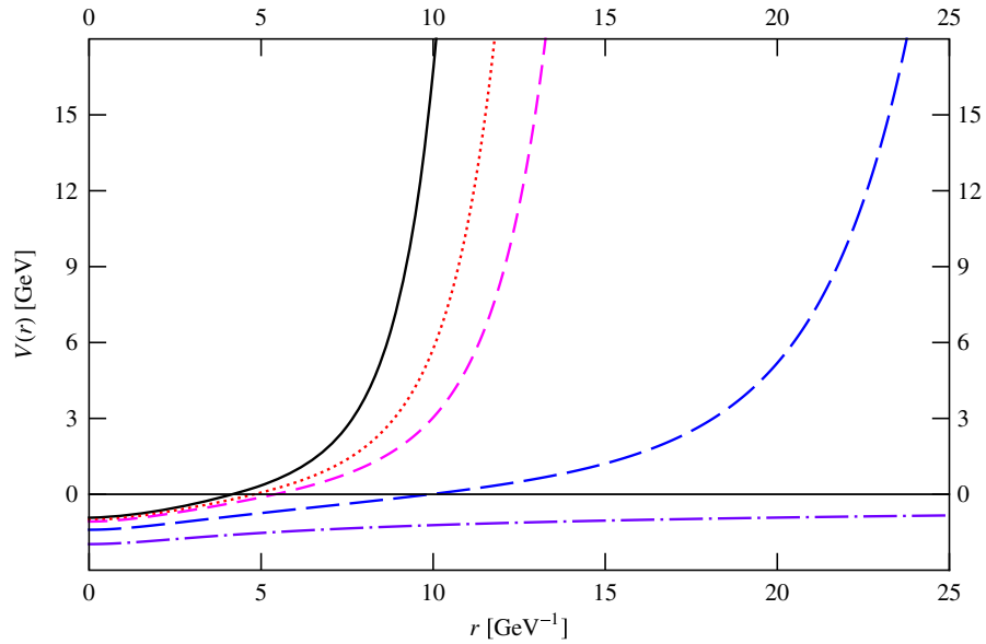
FIG. 4. Configuration-space potential V(r) extracted from the Salpeter equation (2) with interaction-kernel Lorentz structure 2\Gamma \otimes \Gamma = \gamma_\mu \otimes \gamma^\mu + \gamma_5 \otimes \gamma_5 - 1 \otimes 1 , for typical quark-mass value m : m = 0 (black solid line), m = 0.35 GeV (red dotted line), m = 0.5 GeV (magenta short-dashed line), m = 1 GeV (blue long-dashed line), and m = b (violet dot-dashed line).
