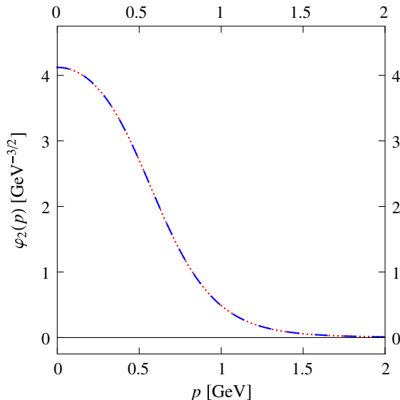
FIG. 2. Comparison of the result of a numerical integration, according to definition (1), of the Bethe-Salpeter amplitude \Phi(\underline{k}, 0) emerging from the quark mass function (8) (red dotted line) with our parametrization (9) defined by the parameter values of Table II (blue dashed line).
