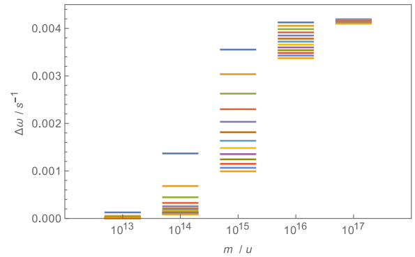
FIG. 4. The resulting frequency spectrum for osmium at T = 100 \text{ mK} at trap frequency \omega_0 = 2\pi \times 10 \text{ s}^{-1} with \Delta n = 1 . At low masses, self-gravity becomes negligible. At high masses all spectral lines are degenerate, shifted by \Delta\omega_{\text{SN}} . The intermediate regime, where a significant splitting appears, spans about 3 orders of magnitude in mass.
