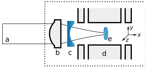
FIG. 3. Schematic of proposed experiment showing (a) optical access, (b) mode-matching lens, (c) concave cavity mirror, (d) ion trap electrode structure, and (e) electrically levitated superconducting disc. The disc acts as a concave cavity mirror and forms an optomechanical cavity with the mirror (c) to read the position of the disc. The apparatus is enclosed in a dilution refrigerator to reduce thermal noises. The longitudinal direction, which will be used to investigate the self-gravity modification of the mechanical harmonic oscillator energy levels, is along the x axis.
