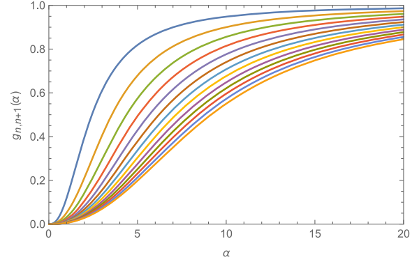
FIG. 2. Plot of the coefficient function g_{n_1 n_2}(\alpha) for the lowest 13 transitions between harmonic oscillator eigenstates with \Delta n = 1 . n increases from top to bottom, with the blue curve belonging to n_1 = 0 . The parameter \alpha characterizes the wave-function width. Small values of \alpha (wide wave functions) correspond to smaller masses (for a given frequency) and therefore weaker self-gravity. In the limit of narrow wave functions (large \alpha ) the lines become degenerate again, with all g_{n_1 n_2} tending to \Delta n = 1 .
