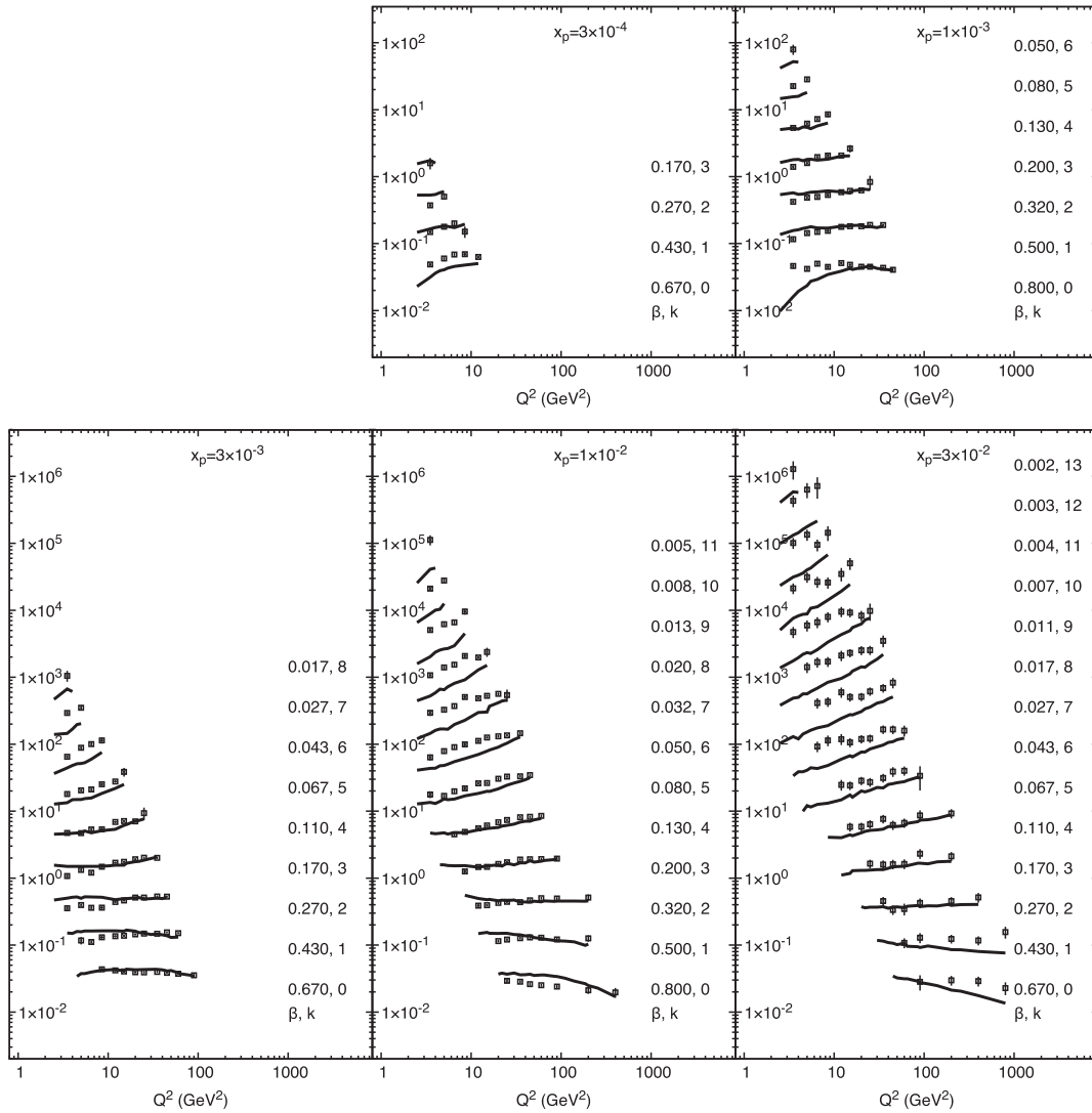
FIG. 6. As in Fig. 3 but with a constant probability of P = 0.103 fitted from this data. We observe that especially at small \beta the resulting diffractive cross section has a significantly different slope with respect to Q^2 , and the description of data is not as good as in the case of the dynamic rescattering model.
