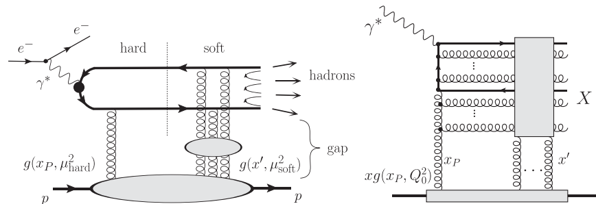
FIG. 1. Illustration of the diffractive DIS process with the hard subprocess matrix element \gamma^* g \rightarrow q\bar{q} with a subsequent rescattering of the q\bar{q} dipole off the target color field (left panel). Schematic diagram of the diffractive DIS process \gamma^* p \rightarrow X + \text{gap} + p accounting for final state rescattering by multiple gluon exchange at x' \ll x_p and perturbative parton shower off initial state parton which builds up the diffractive system X (right panel). The latter can be separated from the leading proton (or small mass system Y ) by a rapidity gap. The final state radiation is not shown as it does not affect the overall kinematics of the X system.
