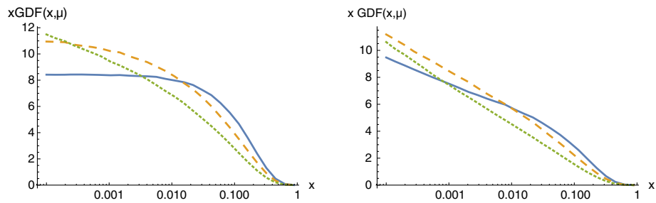
FIG. 8. The gluon density A0 from CASCADE [24] integrated over k_{\perp} at the scales 1, 4 and 8 GeV for the solid, dashed and dotted lines, respectively, is shown in the left panel. The gluon density A1 for the same scales is shown in the right panel. The distribution starts out with a steeper slope at small scales and influences the observable as shown in Fig. 9.
