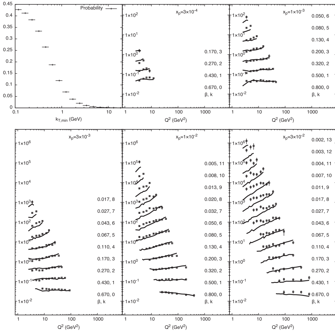
FIG. 10. As in Fig. 3 but showing \sigma_{r,LRG}^D where the diffractive cross section is defined in terms of a large rapidity gap between \eta_{\min} = 4.0 and \eta_{\max} = 6.0 in pseudorapidity.
