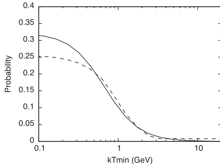
FIG. 7. Dashed line: The fit of a free-form probability function P(k_{\perp \min}) constrained only by the requirement to be in the physically sensible range [0, 1] and to be fairly smooth. Solid line: The probability from the fit of the color screening model as used in Fig. 3 (upper left corner). We note that both methods result in very similar functions for P(k_{\perp \min}) .
