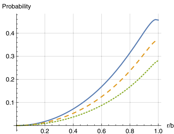
FIG. 2. The screening probability P(r/b) for different values of \alpha_s^{\text{eff}} \in \{0.7, 0.6, 0.5\} (upper to lower curve).
