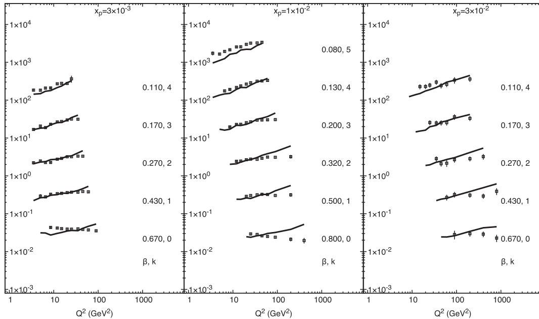
FIG. 9. As in Fig. 3 but using a gluon density xA(x, k_{\perp}, \mu) that increases stronger towards low x already at the starting scale ( A0 in [24]). Only the interesting subset of the kinematic plane is shown. By comparison with Fig. 3 it is seen that \sigma^D(Q^2, \beta, x_p) is at large \beta and large x_p sensitive to the shape of the gluon density at the starting scale.
