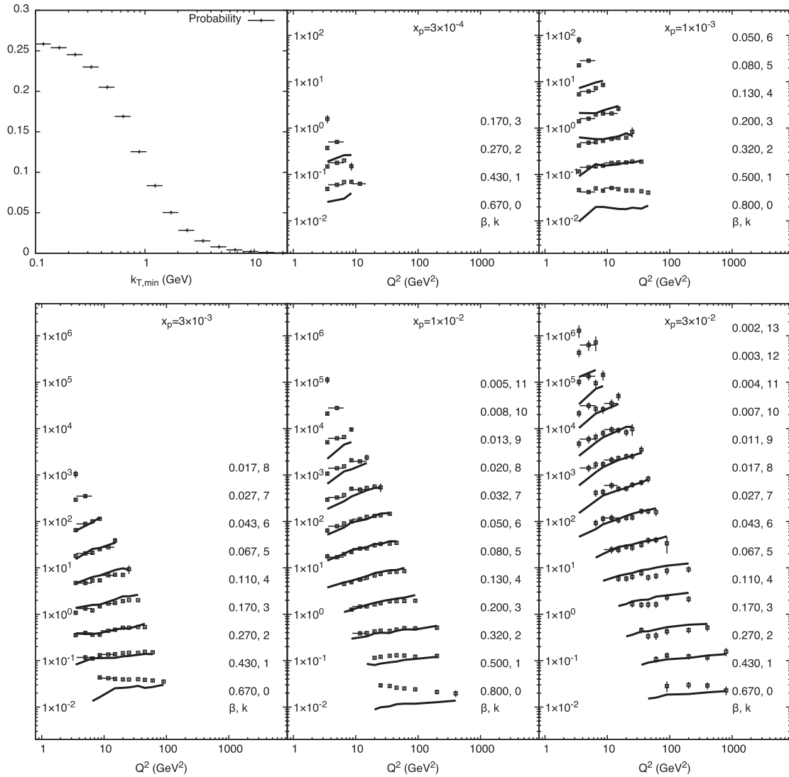
FIG. 5. The reduced diffractive cross section \sigma^D(Q^2, \beta, x_p) as in Fig. 3 but model results using the LEPTO event generator based on matrix elements for all hard processes to order \alpha_s and parton showers based on DGLAP \log Q^2 evolution. The parameters for the dynamic color screening model obtained from the fit against data [28] are k_{\perp 0} = 0.89 GeV and q_{\perp} = 0.66 GeV.
