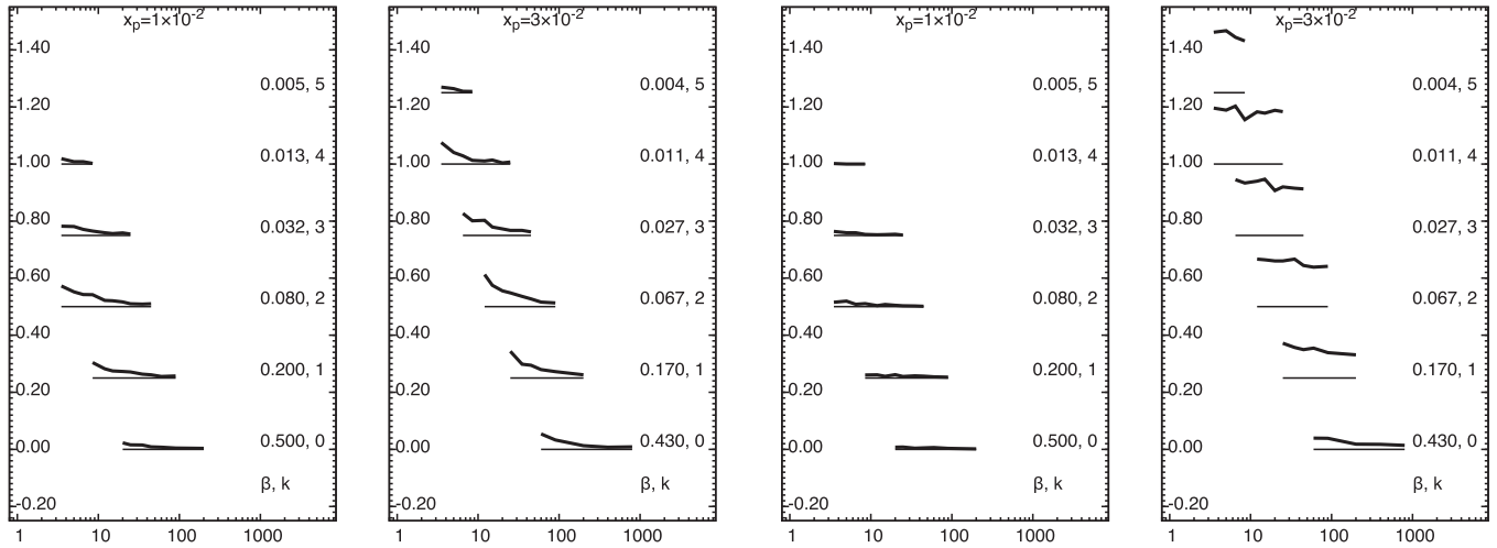
FIG. 11. The fraction of events with a parton level quark with a pseudorapidity in the gap region is shown in the two leftmost plots. The 0% level within the Q^2 range available in the experimental data is indicated by a horizontal thinner line for each row in \beta . The fraction of events with a gluon in the LRG region is shown in the two rightmost plots.
