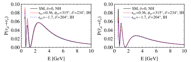
FIG. 4. \nu_\mu \rightarrow \nu_e and \bar{\nu}_\mu \rightarrow \bar{\nu}_e oscillation probabilities at DUNE. The mixing angles and mass-squared differences are the best-fit values in Ref. [12].
