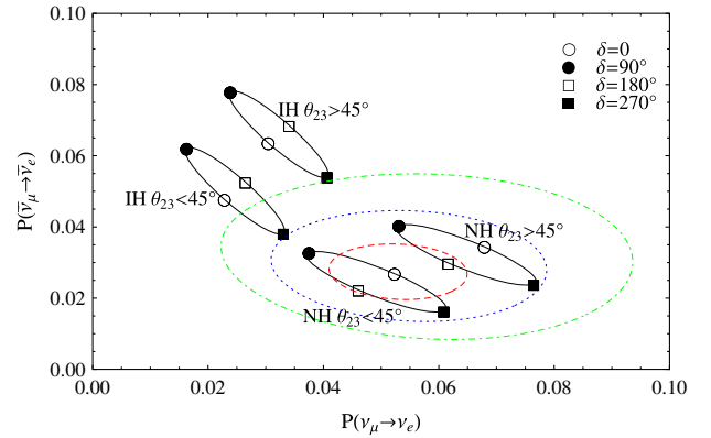
FIG. 1. Biprobability plots ( P(\bar{\nu}_\mu \rightarrow \bar{\nu}_e) versus P(\nu_\mu \rightarrow \nu_e) ) for L = 1300 km and E = 3 GeV. The solid curves show the SM values for fixed mixing angles and varying \delta (one curve for each combination of hierarchy and \theta_{23} octant); the dashed (dotted) [dot-dashed] curves show the values assuming NSI with \epsilon_{e\mu} = 0.05 (0.10) [0.15], and varying \phi_{e\mu} for the NH and first octant with \delta' = 0 . The mixing angles and mass-squared differences are set at their best-fit values from Ref. [12].
