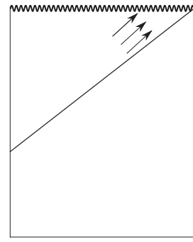
FIG. 11. A state |\Psi_{\text{ex}}\rangle = \tilde{U}|\Psi\rangle corresponding to an equilibrium state |\Psi\rangle excited with a mirror unitary behind the horizon \tilde{U} .
