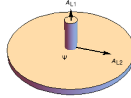
(b) \mathcal{H}_{\Psi_{\text{en}}} in cases with less entanglement. Now the action of “left operators” opens up new directions.
