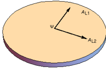
(a) \mathcal{H}_{\Psi_{\text{en}}} where the action of the “left algebra” is entirely contained within the space obtained by acting with the right algebra.
