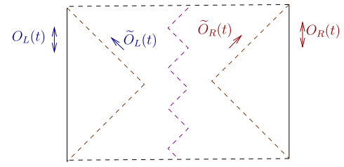
FIG. 14. The dual to the generic entangled state described in Sec. IX C. Simple operators on the right \mathcal{O}_R(t) and left are not correlated. This is indicated by the jagged broken line in the middle and there is no geometric wormhole. But both sides see a smooth horizon with the emergence of new mirror operators behind the horizon.
