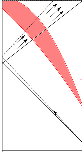
FIG. 16. Tracing the mirrors back to their origin on the boundary is difficult because of the trans-Planckian problem. However, even neglecting this issue does not help in constructing state-independent operators because of the fat tail in the inner product of different solutions.
