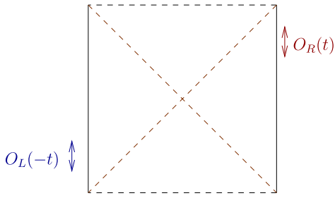
FIG. 13. The standard wormhole described in Sec. IX B: operators on the right \mathcal{O}_R(t) are entangled with left operator \mathcal{O}_L(-t) .
