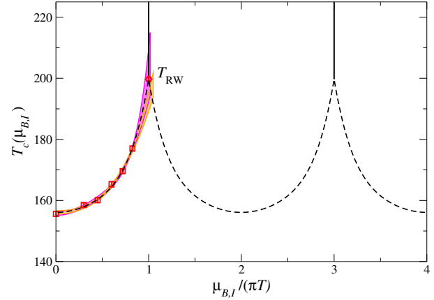
FIG. 9. Phase diagram of QCD in the presence of an imaginary baryon chemical potential obtained from numerical simulations on N_t = 8 lattices alone. Bands denote fits to polynomials in \mu_B^2 : the orange (longer) band is obtained using terms up to order \mu_B^4 and the violet (shorter) one using up to \mu_B^6 terms.
