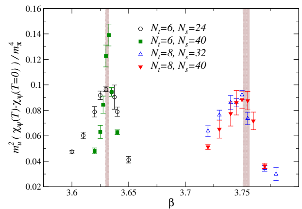
FIG. 10. Renormalized light chiral susceptibility on N_t = 6 and 8 lattices. The vertical bands denote the position of the RW endpoint on lattices of the corresponding temporal extent.
