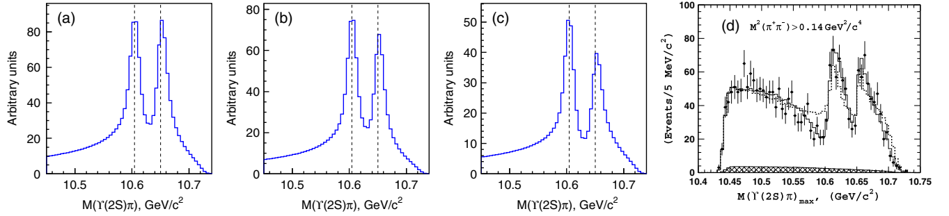
FIG. 7. Plots (a), (b), and (c) are for the predicted line shapes of the Z_b(10610) and Z_b(10650) in the \pi\Upsilon(2S) channel for fits A, B, and C, respectively. To guide the eye, as plot (d), we also show the corresponding experimental figure adapted from Ref. [46]. Notice that the behavior of the line shape below the left shoulder of the lower peak is influenced by the effects which lie beyond the scope of the present paper and will be addressed in future publications. Notice also that the presence of the nonresonant background in the experimental figure does not allow its direct comparison with the predicted line shapes.
