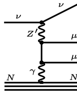
FIG. 10. Neutrino trident process that leads to constraints on the Z' coupling strength to neutrinos-muons, namely M_{Z'}/g_{\nu\mu} \gtrsim 750 GeV.
