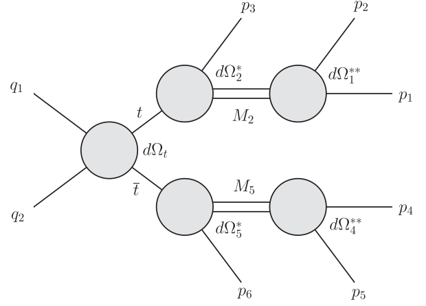
FIG. 1. Kinematics for gg \rightarrow t\bar{t} \rightarrow (b\bar{b}c)(\bar{b}\ell\bar{\nu}) [10]. The definitions of the various angles and invariant masses are identical to those given in Ref. [7]; these definitions are reproduced here for convenience. \Omega_1^{**} denotes the direction of \vec{p}_1^{**} in the rest frame of M_2 , relative to the direction of \vec{p}_1^* + \vec{p}_2^* , where M_2^2 = (p_1 + p_2)^2 . Similarly, \Omega_2^* denotes the direction of (\vec{p}_1^* + \vec{p}_2^*) in the t rest frame, relative to the direction of \vec{p}_t in the t\bar{t} rest frame. \Omega_t denotes the direction of \vec{p}_t relative to \vec{q}_1 , also in the t\bar{t} rest frame. The solid angles \Omega_4^{**} and \Omega_5^* are defined analogously to \Omega_1^{**} and \Omega_2^* , respectively, and M_5^2 = (p_4 + p_5)^2 . In this work we take p_1 = p_c , p_2 = p_b , p_3 = p_{\bar{b}_1} , p_4 = p_{\bar{b}} , p_5 = p_{\bar{\nu}_\ell} and p_6 = p_\ell .
