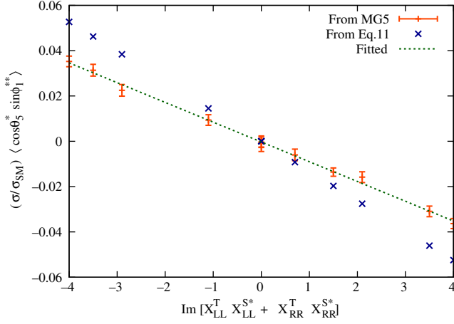
FIG. 2. Plot of (\sigma/\sigma_{\text{SM}})\langle\cos\theta_5^* \sin\phi_1^{**}\rangle as a function of \text{Im}[X_{LL}^T X_{LL}^{S*} + X_{RR}^T X_{RR}^{S*}] for various combinations of NP parameters. As is evident from the plot, the simulated data have a linear dependence on \text{Im}[X_{LL}^T X_{LL}^{S*} + X_{RR}^T X_{RR}^{S*}] , as in Eq. (11), even though Eq. (11) was derived under several simplifying assumptions.
