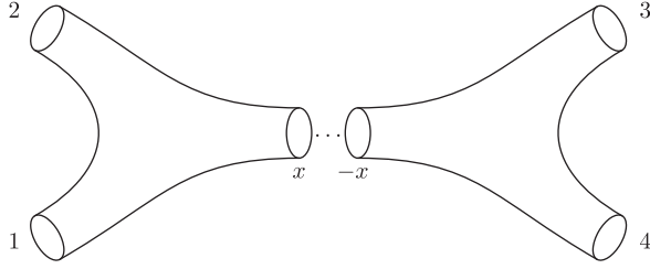
FIG. 1. The factorization of the tree-level four-point amplitude in the massless pole s_{12} in terms of three-point amplitudes. This condition was used to fix the normalization constant \kappa^2 = \frac{\pi e^{2\lambda}}{\alpha^2} in Eq. (A7).
