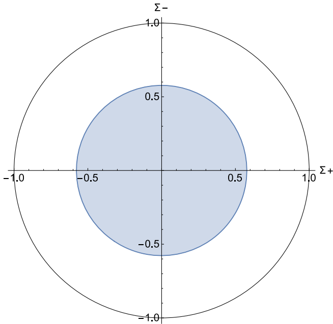
FIG. 1. A plot of the Kasner circle \Sigma_+^2 + \Sigma_-^2 = 1 . For eternal inflation to occur, the anisotropy variables must take on values (\Sigma_+, \Sigma_-) within the shaded region.
