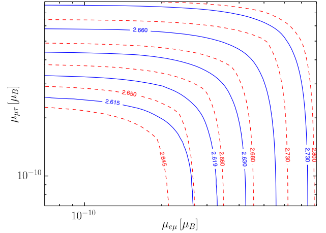
FIG. 8 (color online). Contours of constant 10^5 \times D/H in the \mu_{\mu\tau} versus \mu_{e\mu} plane. The solid contours correspond to \mu_{e\tau} = 10^{-10} \mu_B and the dashed contours correspond to \mu_{e\tau} = 4.9 \times 10^{-10} \mu_B .
