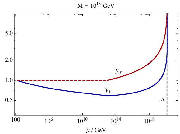
FIG. 1 (color online). The RG evolutions of the top (solid) and neutrino (dashed) HY couplings with contributions from right-handed neutrinos for renormalization scales above the neutrino Majorana mass; \mu > M = 10^{13} GeV.
