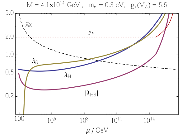
FIG. 4 (color online). The RG evolution for the quartic couplings in the communicated CW setup. Choosing the active neutrino mass and Majorana mass determines the compositeness scale, where the quartics are given values such that \lambda_H = |\lambda_{HS}| = \lambda_S \approx y_\nu^2 at this scale. The final assumption is that g_X(m_Z) = 5.5 , which determines the IR behavior and symmetry breaking pattern. The evolution shown above yields v \approx 174 GeV and m_H \approx 126 GeV.
