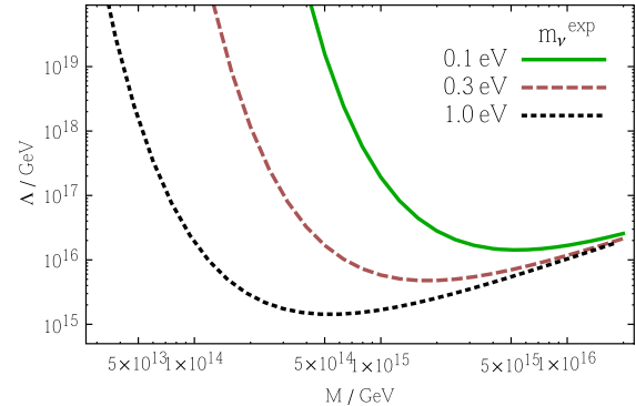
FIG. 2 (color online). Numerical results displaying the relation between the Majorana mass and the scale associated with the Landau pole for the neutrino HY coupling for different values of the neutrino mass.
