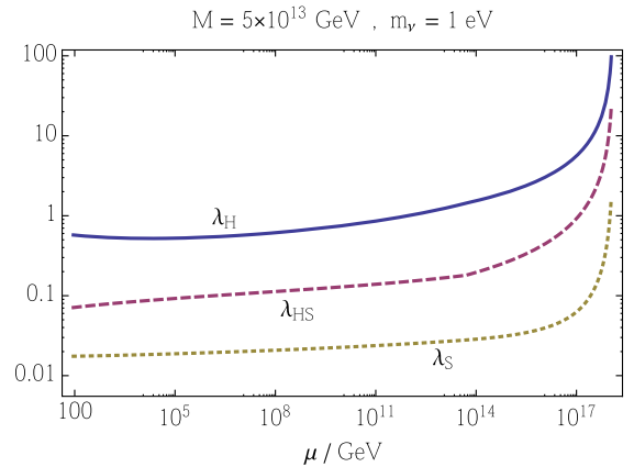
FIG. 3 (color online). The RG evolution for the quartic couplings for a specific choice of initial conditions at the UV scale. The IR phenomenology features a large quartic for the Higgs, while the effective coupling leads to a light Higgs mass m_H \sim 130 GeV.
